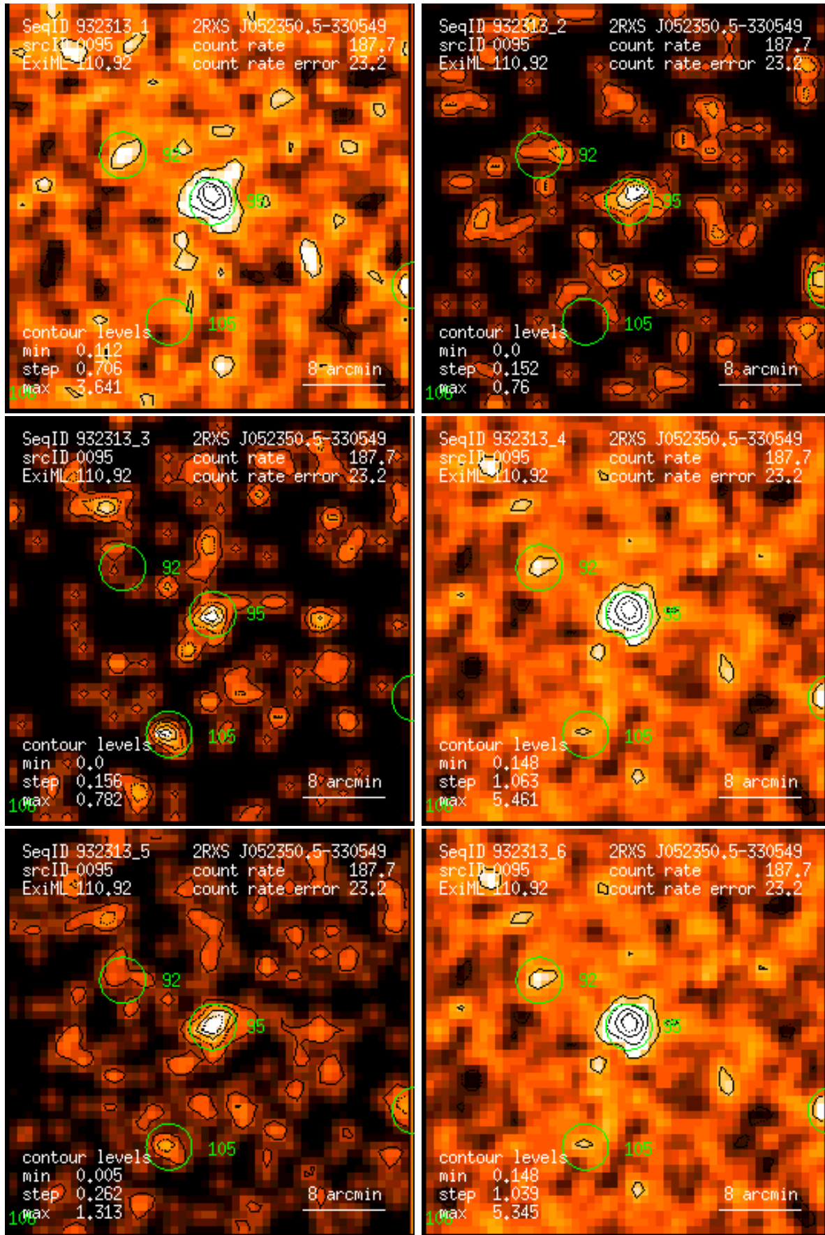
Figure 95: RASS 932313: detection 0095: band rate images, Gaussian filter: (1) PSPC channels 11 – 41, (2) 52 – 90, (3) 91 – 201, (4) 11 – 235, (5) 52 – 201, (6) 11 – 201. Broad band rates in counts/ks. Band rate contour levels in counts/ks/arcmin 2 .
