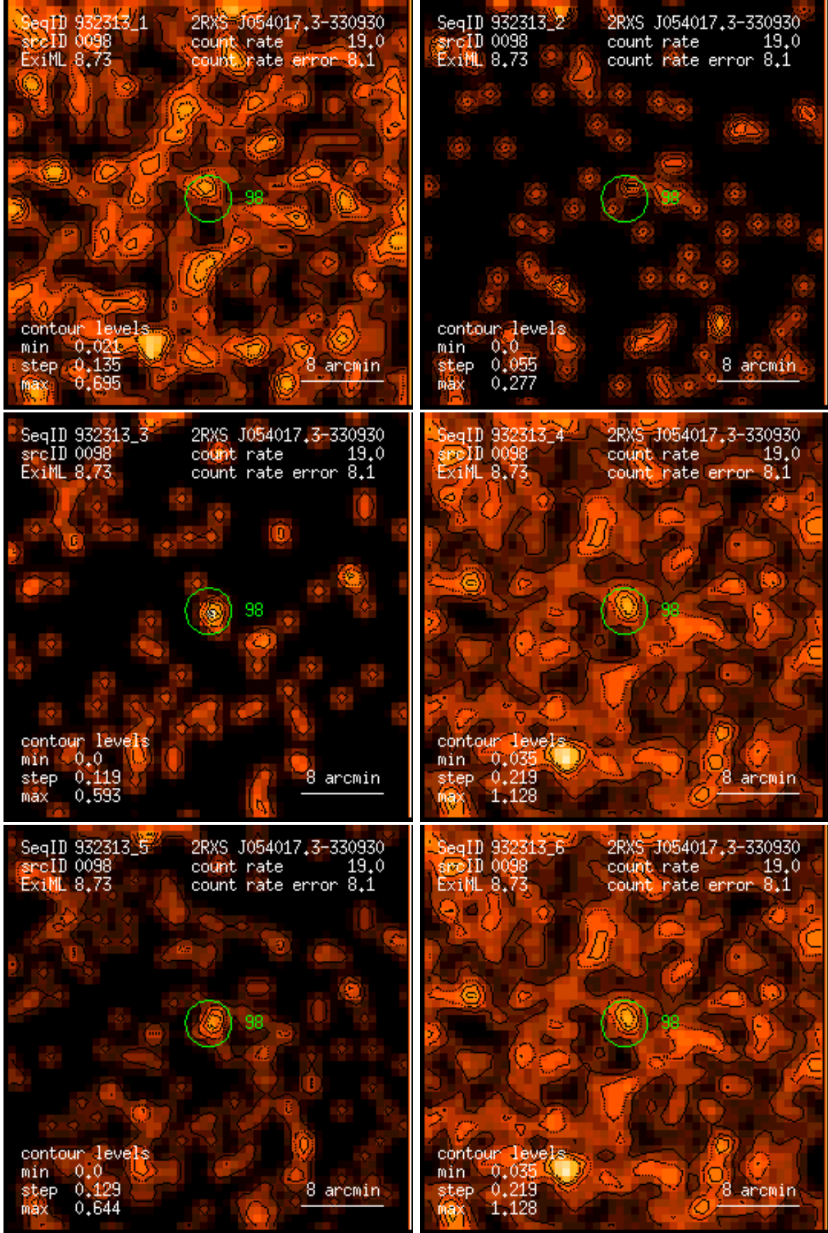
Figure 98: RASS 932313: detection 0098: band rate images, Gaussian filter: (1) PSPC channels 11 – 41, (2) 52 – 90, (3) 91 – 201, (4) 11 – 235, (5) 52 – 201, (6) 11 – 201. Broad band rates in counts/ks. Band rate contour levels in counts/ks/arcmin 2 .
