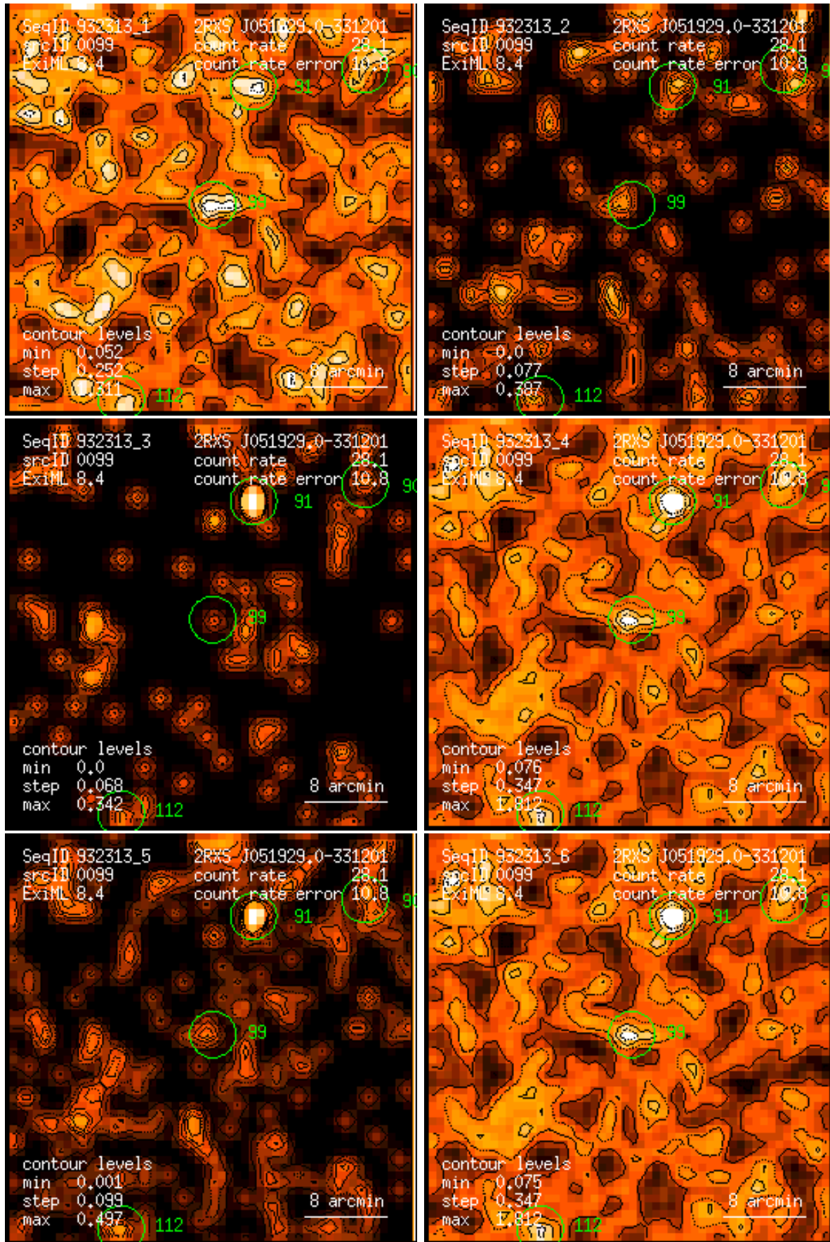
Figure 99: RASS 932313: detection 0099: band rate images, Gaussian filter: (1) PSPC channels 11 – 41, (2) 52 – 90, (3) 91 – 201, (4) 11 – 235, (5) 52 – 201, (6) 11 – 201. Broad band rates in counts/ks. Band rate contour levels in counts/ks/arcmin 2 .
