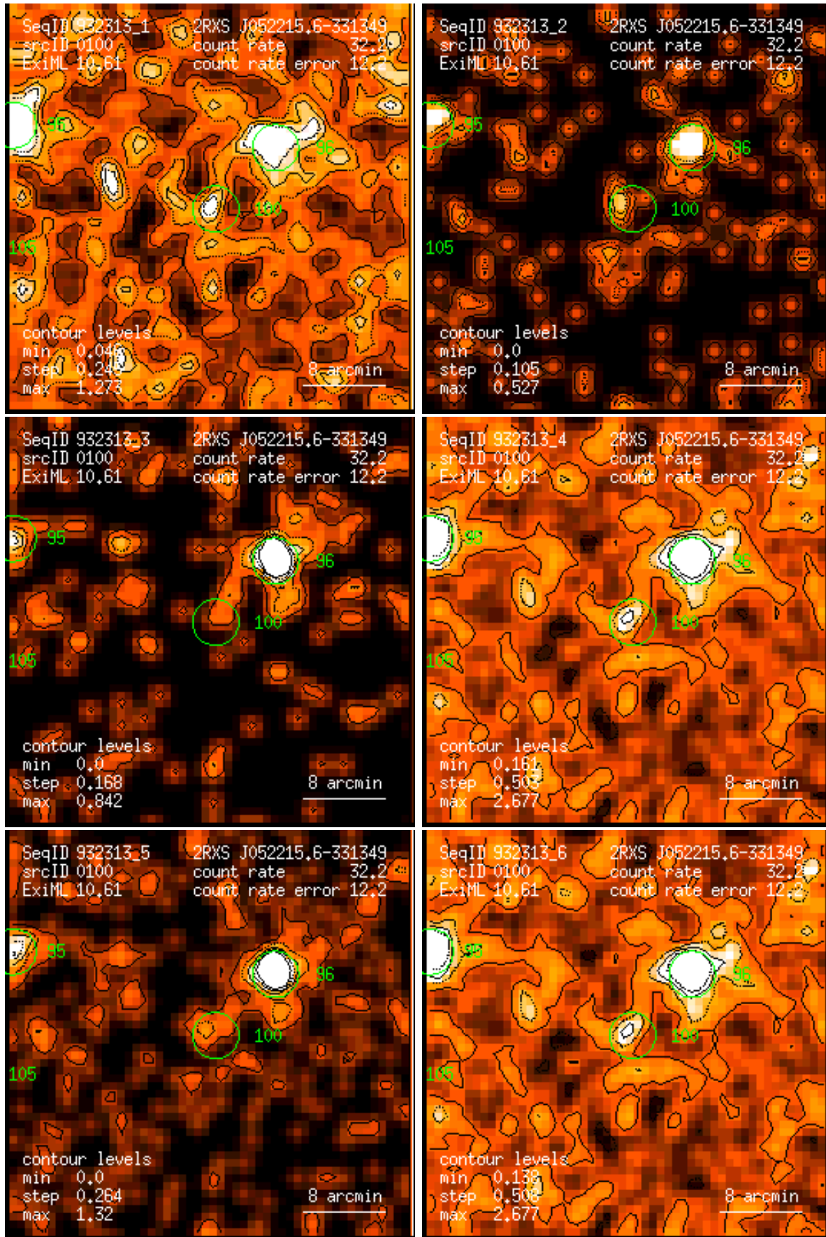
Figure 100: RASS 932313: detection 0100: band rate images, Gaussian filter: (1) PSPC channels 11 – 41, (2) 52 – 90, (3) 91 – 201, (4) 11 – 235, (5) 52 – 201, (6) 11 – 201. Broad band rates in counts/ks. Band rate contour levels in counts/ks/arcmin 2 .
