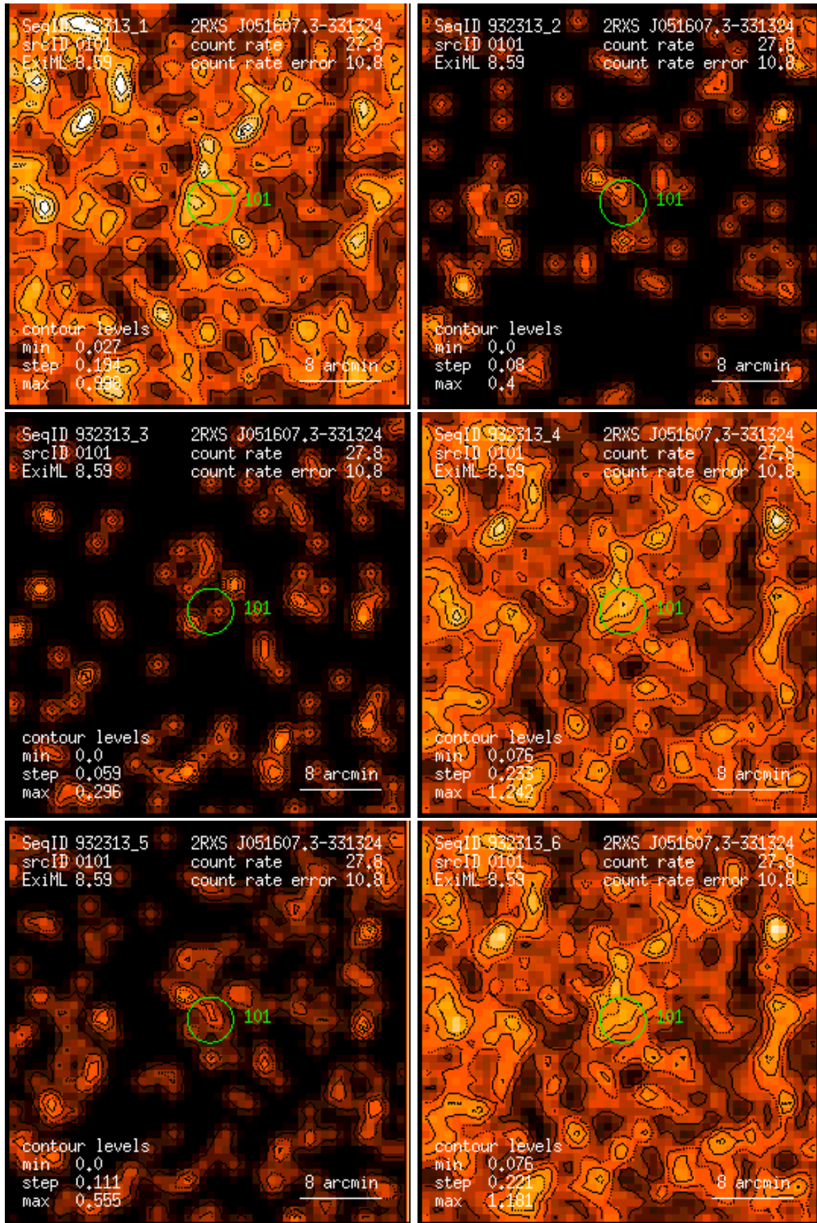
Figure 101: RASS 932313: detection 0101: band rate images, Gaussian filter: (1) PSPC channels 11 – 41, (2) 52 – 90, (3) 91 – 201, (4) 11 – 235, (5) 52 – 201, (6) 11 – 201. Broad band rates in counts/ks. Band rate contour levels in counts/ks/arcmin 2 .
