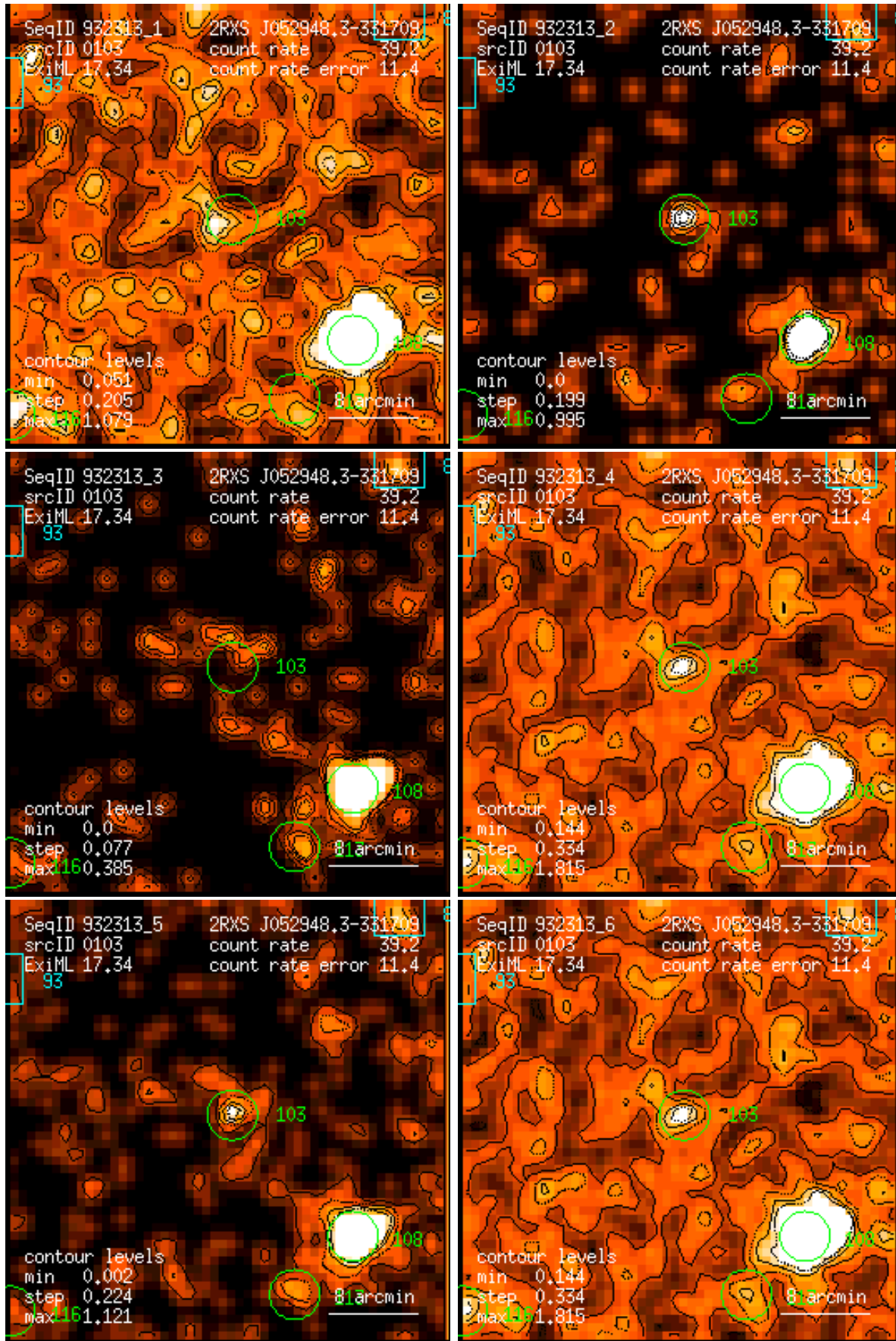
Figure 103: RASS 932313: detection 0103: band rate images, Gaussian filter: (1) PSPC channels 11 – 41, (2) 52 – 90, (3) 91 – 201, (4) 11 – 235, (5) 52 – 201, (6) 11 – 201. Broad band rates in counts/ks. Band rate contour levels in counts/ks/arcmin 2 .
