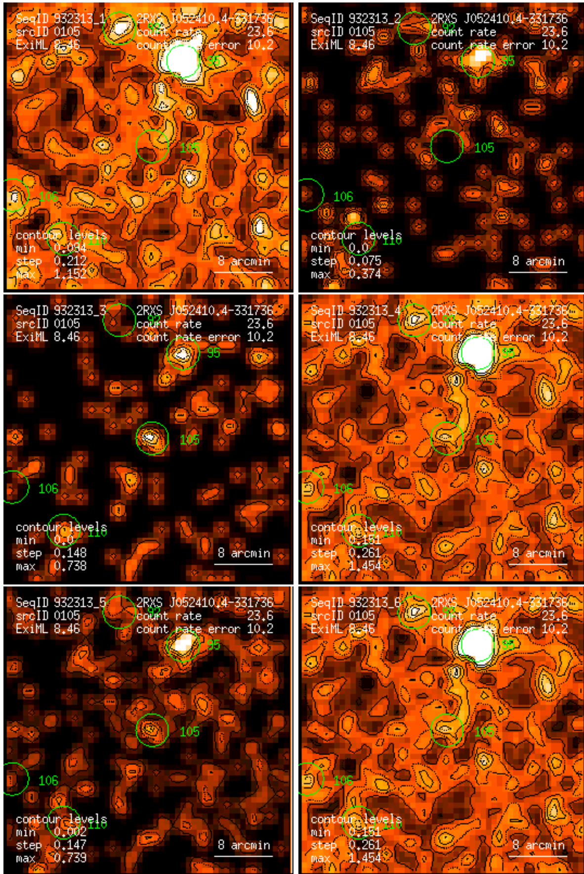
Figure 105: RASS 932313: detection 0105: band rate images, Gaussian filter: (1) PSPC channels 11 – 41, (2) 52 – 90, (3) 91 – 201, (4) 11 – 235, (5) 52 – 201, (6) 11 – 201. Broad band rates in counts/ks. Band rate contour levels in counts/ks/arcmin 2 .
