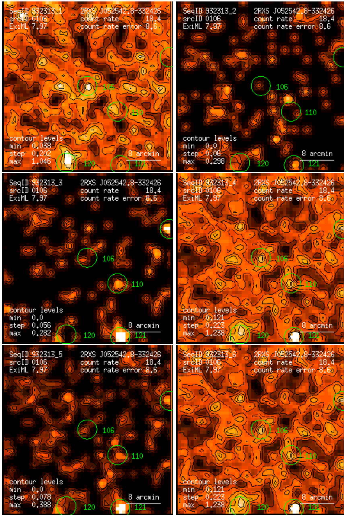
Figure 106: RASS 932313: detection 0106: band rate images, Gaussian filter: (1) PSPC channels 11 – 41, (2) 52 – 90, (3) 91 – 201, (4) 11 – 235, (5) 52 – 201, (6) 11 – 201. Broad band rates in counts/ks. Band rate contour levels in counts/ks/arcmin 2 .
