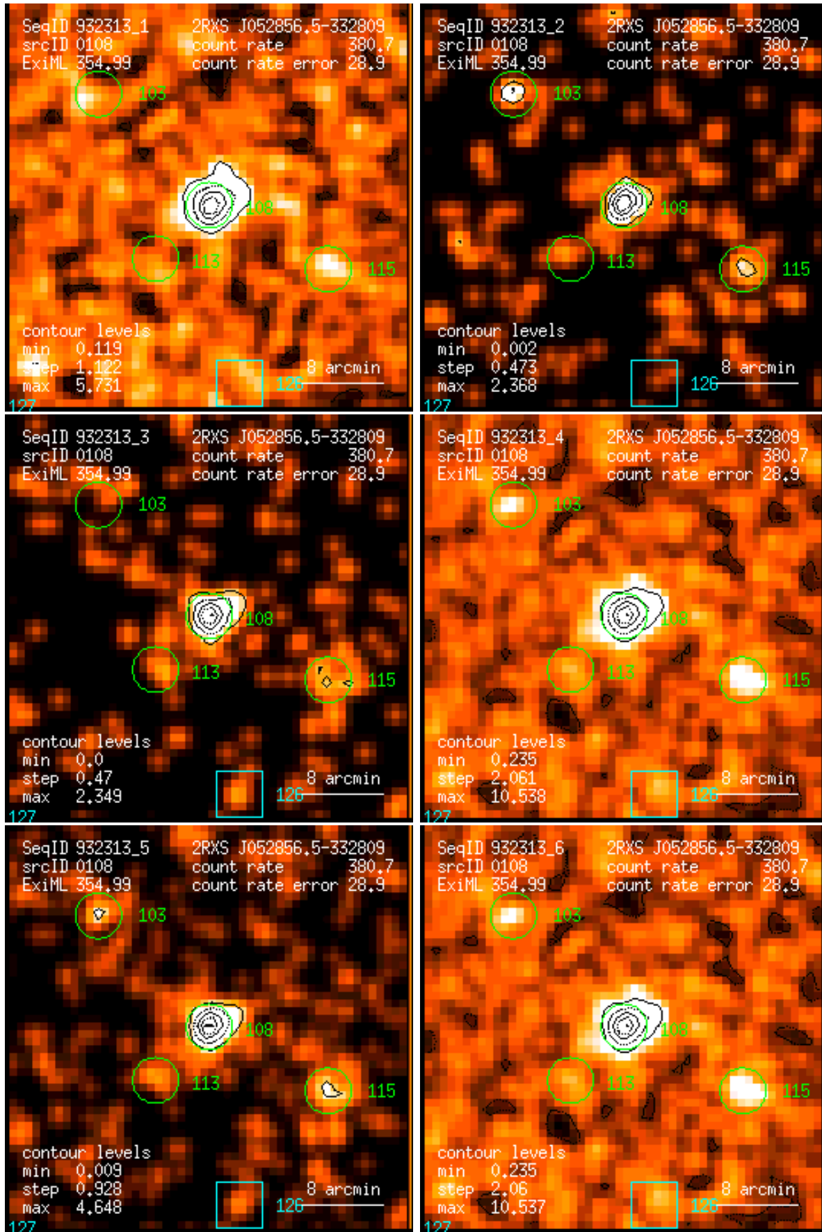
Figure 108: RASS 932313: detection 0108: band rate images, Gaussian filter: (1) PSPC channels 11 – 41, (2) 52 – 90, (3) 91 – 201, (4) 11 – 235, (5) 52 – 201, (6) 11 – 201. Broad band rates in counts/ks. Band rate contour levels in counts/ks/arcmin 2 .
