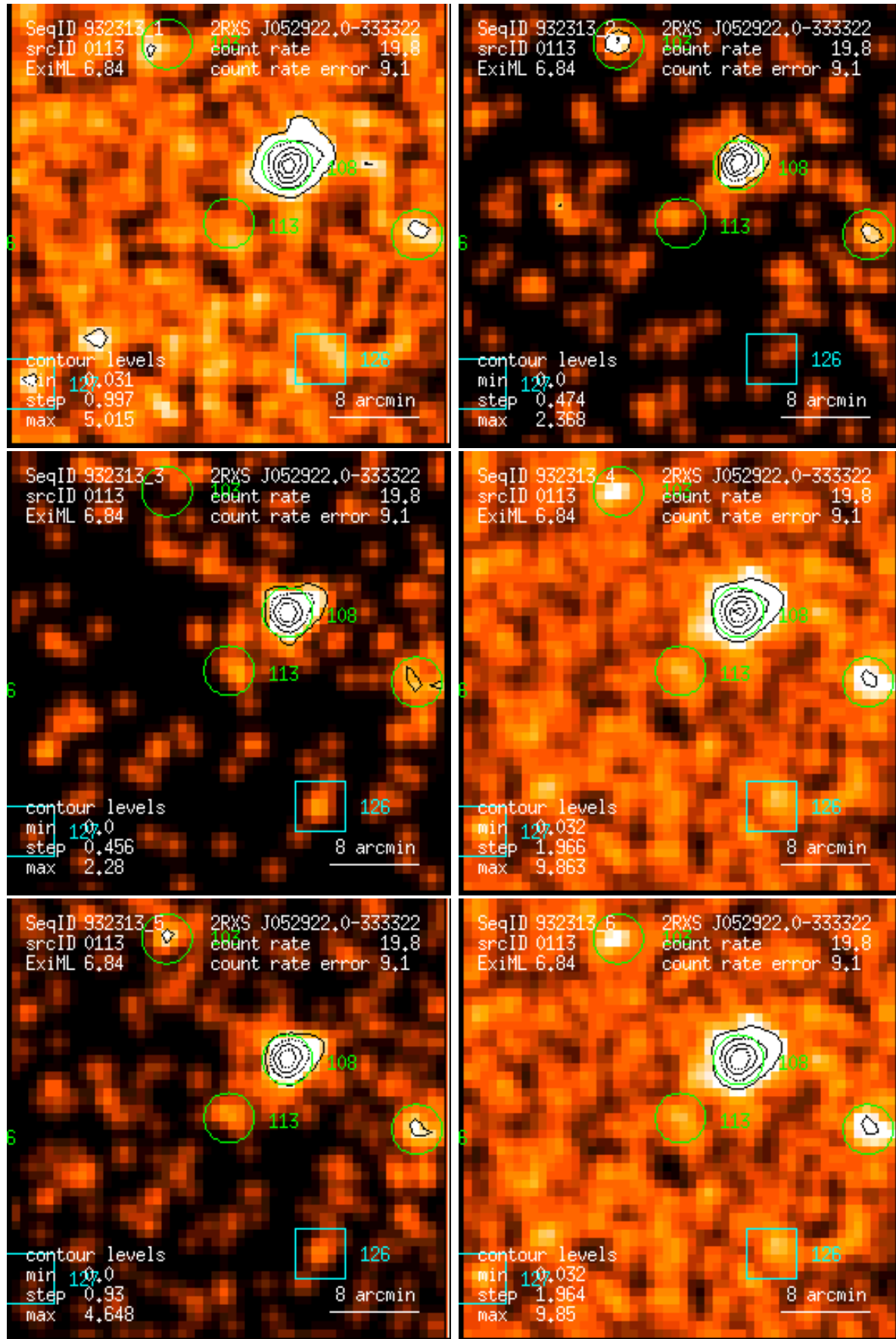
Figure 113: RASS 932313: detection 0113: band rate images, Gaussian filter: (1) PSPC channels 11 – 41, (2) 52 – 90, (3) 91 – 201, (4) 11 – 235, (5) 52 – 201, (6) 11 – 201. Broad band rates in counts/ks. Band rate contour levels in counts/ks/arcmin 2 .
