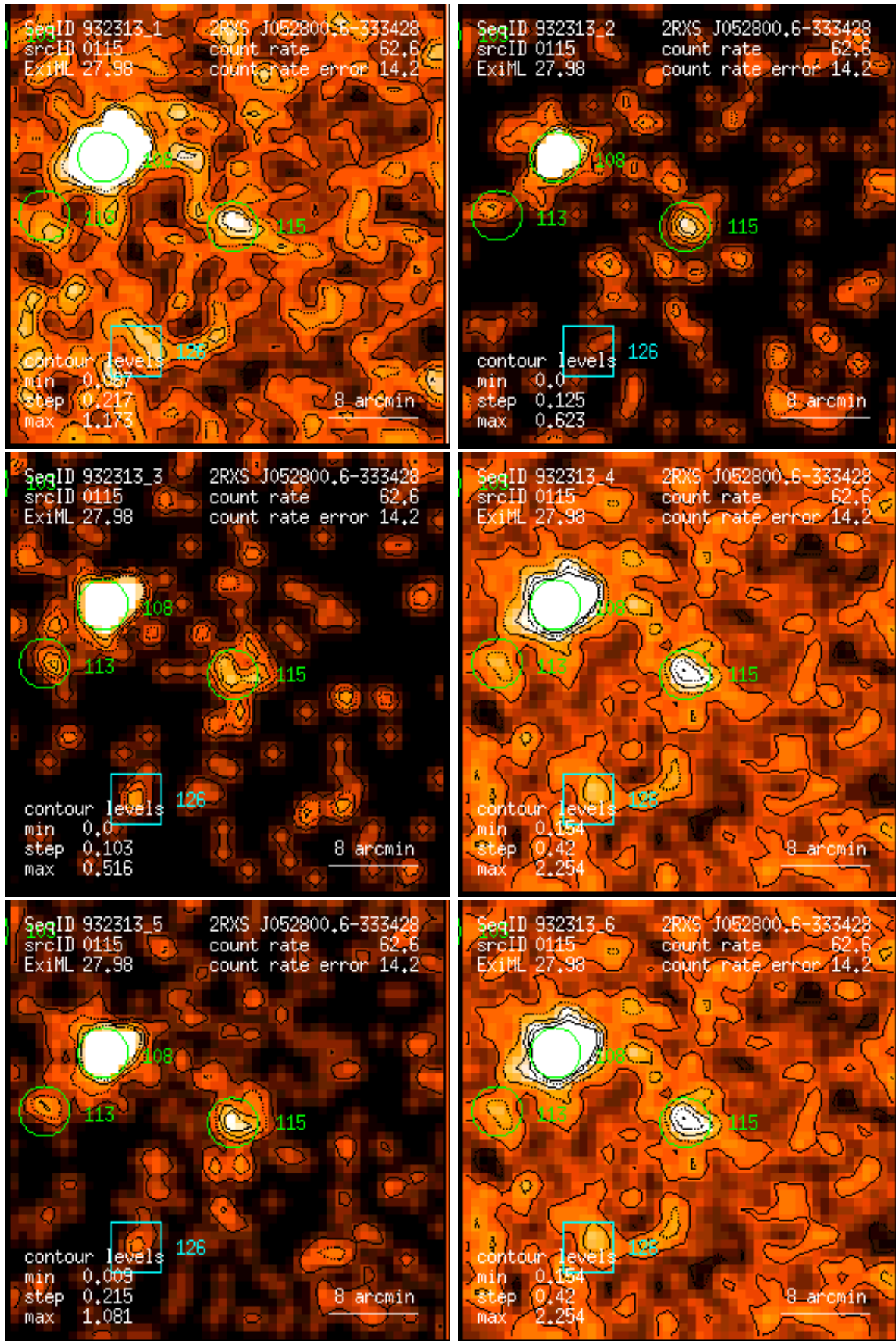
Figure 115: RASS 932313: detection 0115: band rate images, Gaussian filter: (1) PSPC channels 11 – 41, (2) 52 – 90, (3) 91 – 201, (4) 11 – 235, (5) 52 – 201, (6) 11 – 201. Broad band rates in counts/ks. Band rate contour levels in counts/ks/arcmin 2 .
