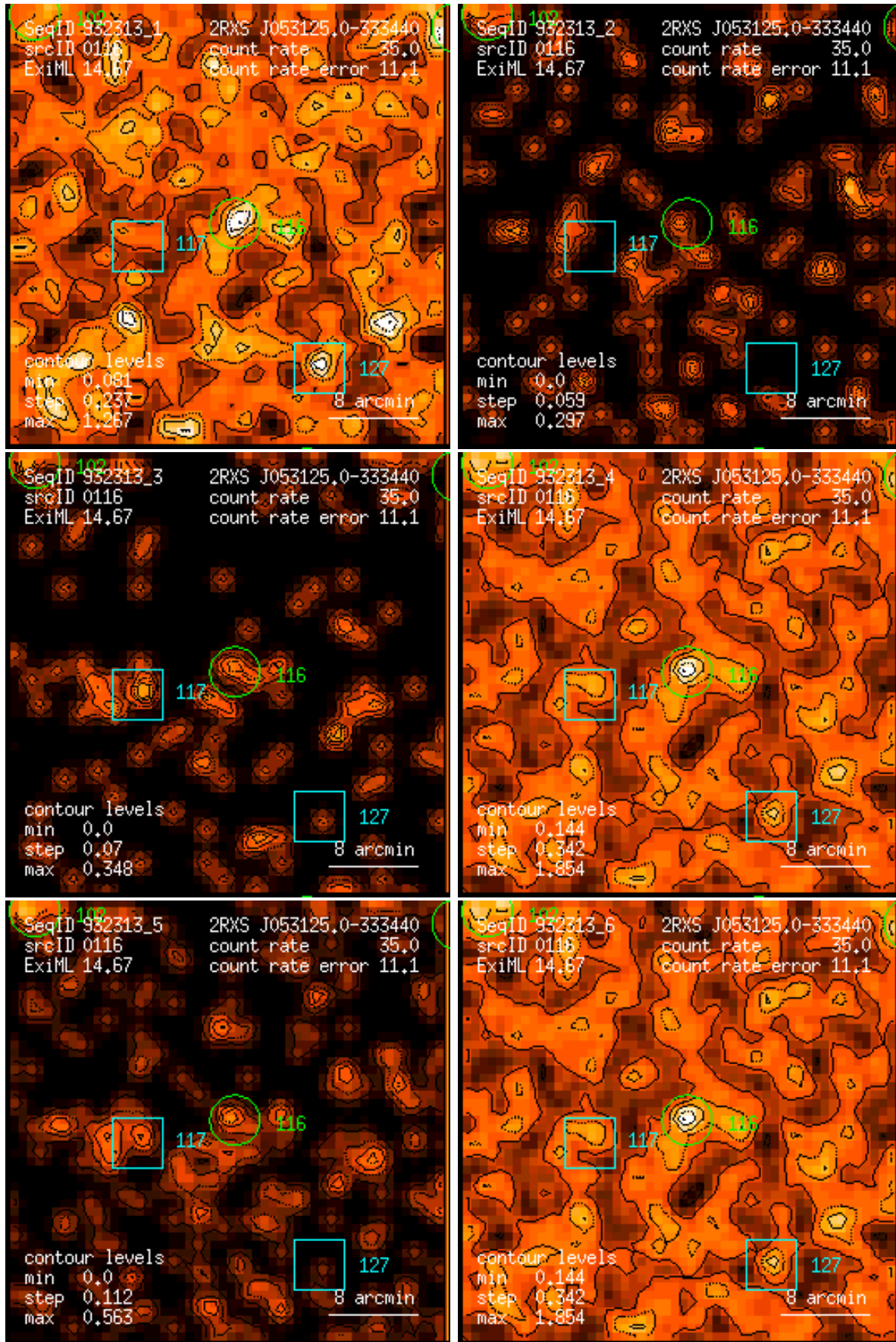
Figure 116: RASS 932313: detection 0116: band rate images, Gaussian filter: (1) PSPC channels 11 – 41, (2) 52 – 90, (3) 91 – 201, (4) 11 – 235, (5) 52 – 201, (6) 11 – 201. Broad band rates in counts/ks. Band rate contour levels in counts/ks/arcmin 2 .
