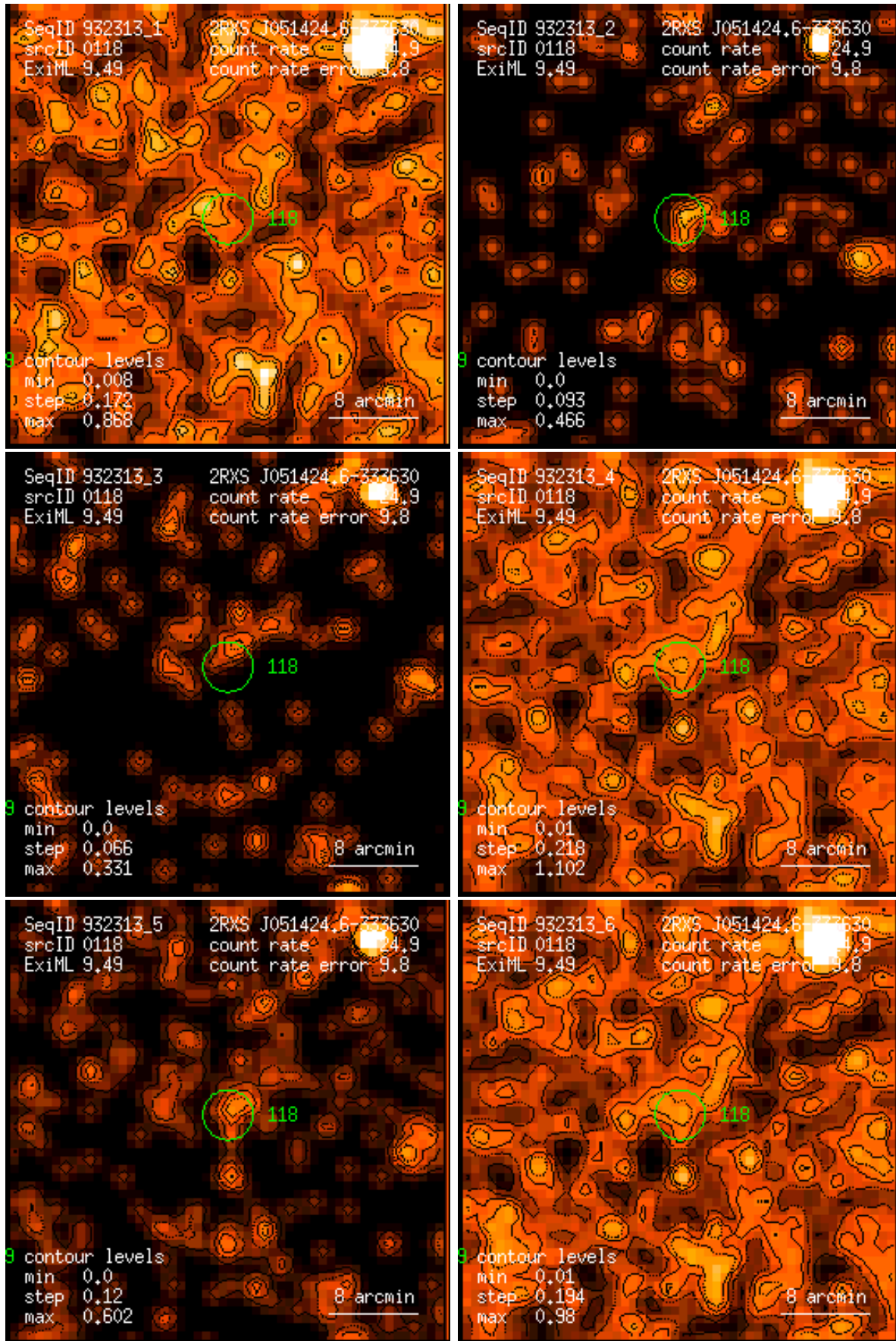
Figure 118: RASS 932313: detection 0118: band rate images, Gaussian filter: (1) PSPC channels 11 – 41, (2) 52 – 90, (3) 91 – 201, (4) 11 – 235, (5) 52 – 201, (6) 11 – 201. Broad band rates in counts/ks. Band rate contour levels in counts/ks/arcmin 2 .
