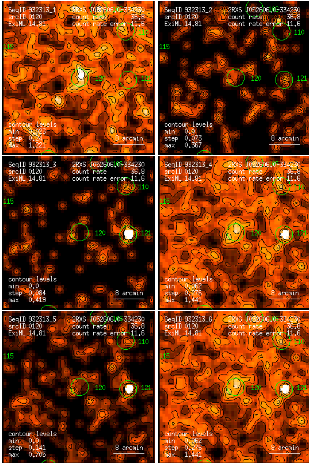
Figure 120: RASS 932313: detection 0120: band rate images, Gaussian filter: (1) PSPC channels 11 – 41, (2) 52 – 90, (3) 91 – 201, (4) 11 – 235, (5) 52 – 201, (6) 11 – 201. Broad band rates in counts/ks. Band rate contour levels in counts/ks/arcmin 2 .
