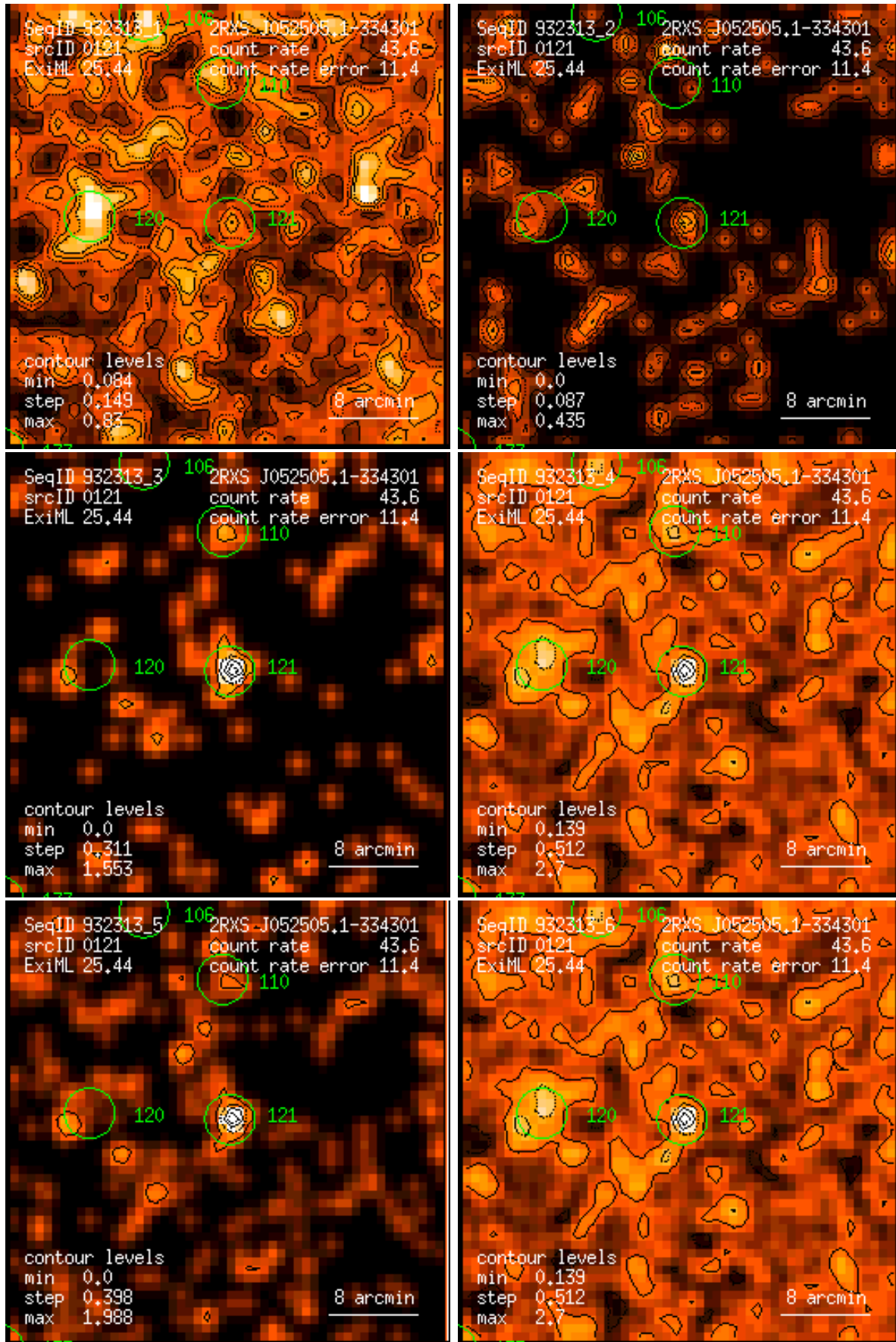
Figure 121: RASS 932313: detection 0121: band rate images, Gaussian filter: (1) PSPC channels 11 – 41, (2) 52 – 90, (3) 91 – 201, (4) 11 – 235, (5) 52 – 201, (6) 11 – 201. Broad band rates in counts/ks. Band rate contour levels in counts/ks/arcmin 2 .
