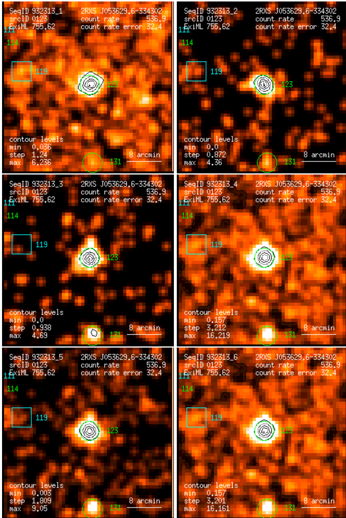
Figure 123: RASS 932313: detection 0123: band rate images, Gaussian filter: (1) PSPC channels 11 – 41, (2) 52 – 90, (3) 91 – 201, (4) 11 – 235, (5) 52 – 201, (6) 11 – 201. Broad band rates in counts/ks. Band rate contour levels in counts/ks/arcmin 2 .
