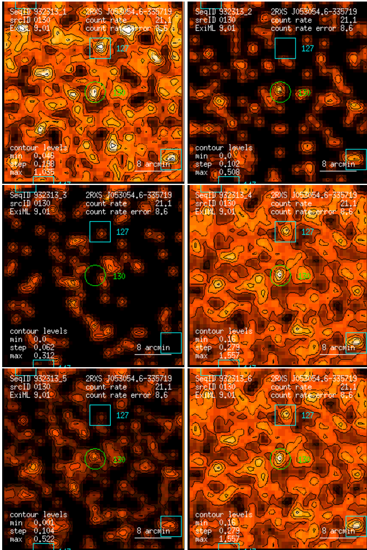
Figure 130: RASS 932313: detection 0130: band rate images, Gaussian filter: (1) PSPC channels 11 – 41, (2) 52 – 90, (3) 91 – 201, (4) 11 – 235, (5) 52 – 201, (6) 11 – 201. Broad band rates in counts/ks. Band rate contour levels in counts/ks/arcmin 2 .
