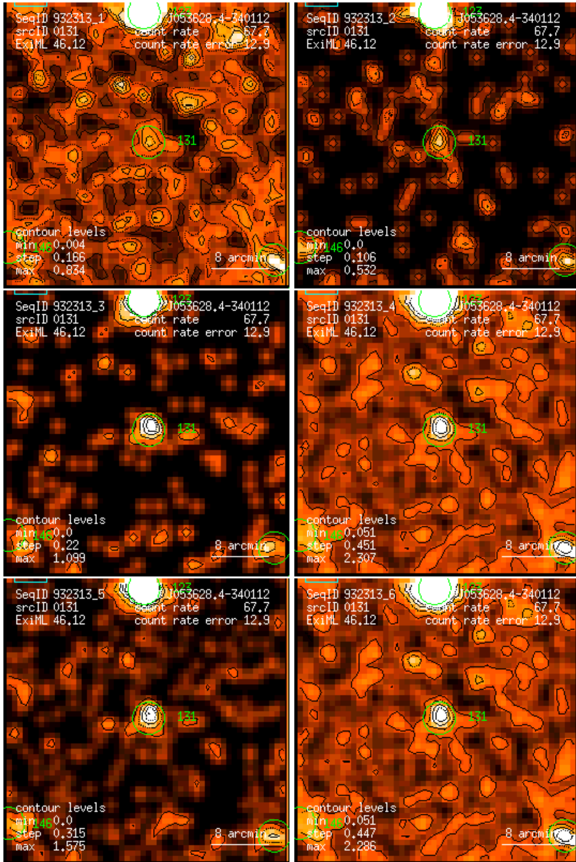
Figure 131: RASS 932313: detection 0131: band rate images, Gaussian filter: (1) PSPC channels 11 – 41, (2) 52 – 90, (3) 91 – 201, (4) 11 – 235, (5) 52 – 201, (6) 11 – 201. Broad band rates in counts/ks. Band rate contour levels in counts/ks/arcmin 2 .
