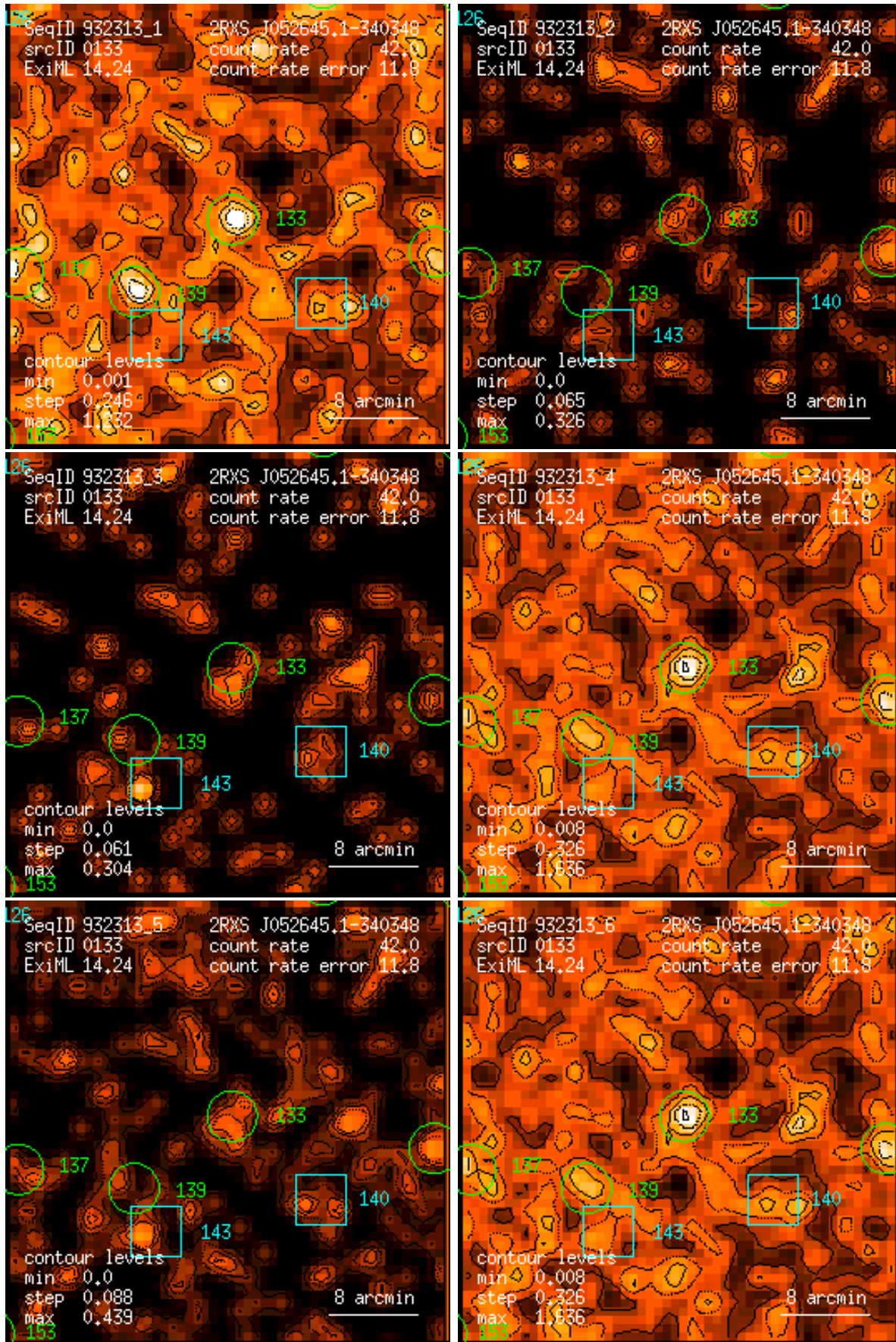
Figure 133: RASS 932313: detection 0133: band rate images, Gaussian filter: (1) PSPC channels 11 – 41, (2) 52 – 90, (3) 91 – 201, (4) 11 – 235, (5) 52 – 201, (6) 11 – 201. Broad band rates in counts/ks. Band rate contour levels in counts/ks/arcmin 2 .
