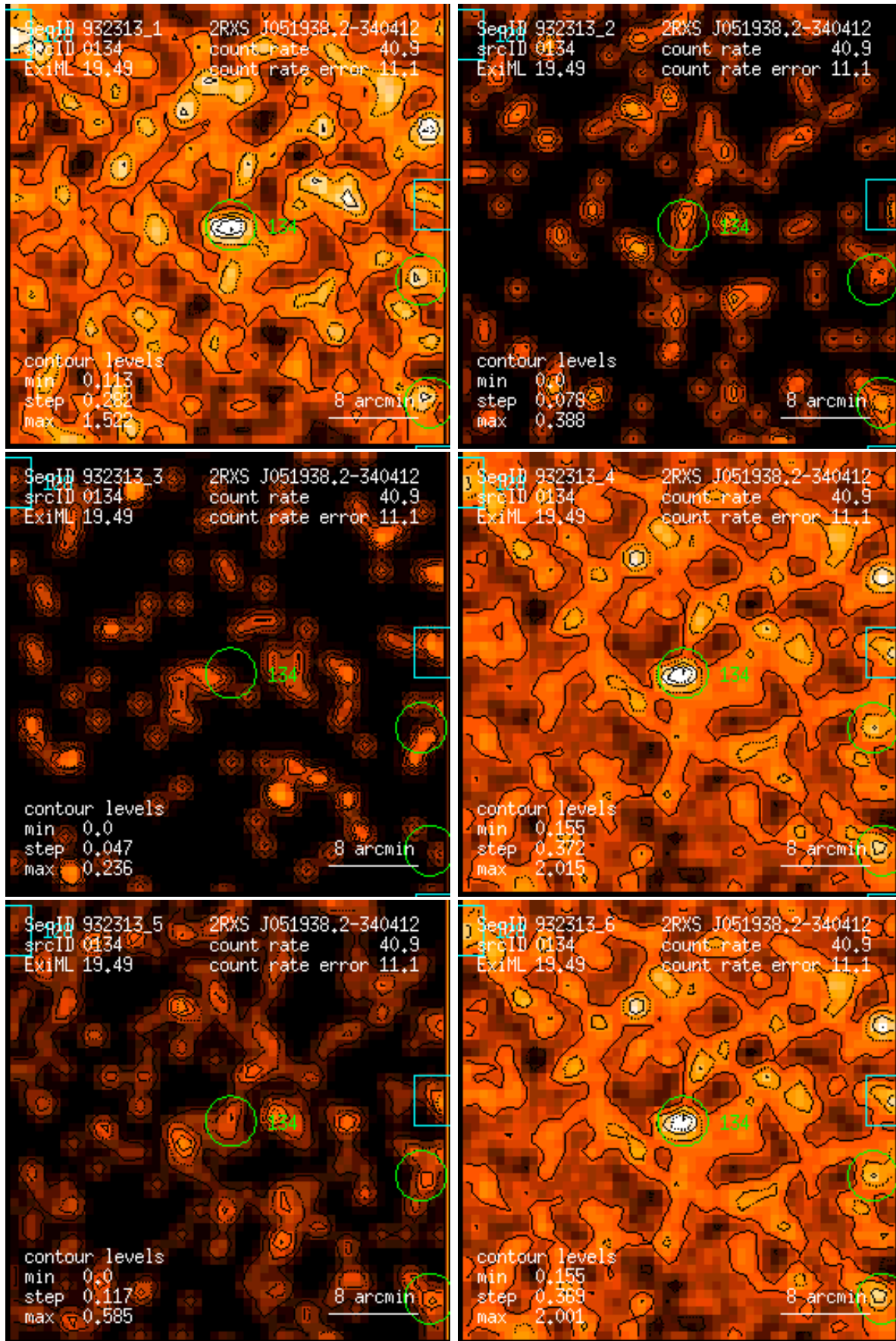
Figure 134: RASS 932313: detection 0134: band rate images, Gaussian filter: (1) PSPC channels 11 – 41, (2) 52 – 90, (3) 91 – 201, (4) 11 – 235, (5) 52 – 201, (6) 11 – 201. Broad band rates in counts/ks. Band rate contour levels in counts/ks/arcmin 2 .
