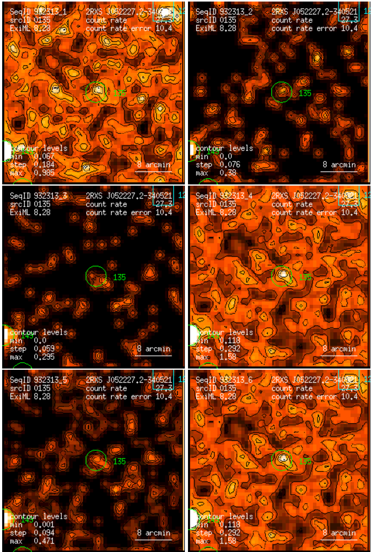
Figure 135: RASS 932313: detection 0135: band rate images, Gaussian filter: (1) PSPC channels 11 – 41, (2) 52 – 90, (3) 91 – 201, (4) 11 – 235, (5) 52 – 201, (6) 11 – 201. Broad band rates in counts/ks. Band rate contour levels in counts/ks/arcmin 2 .
