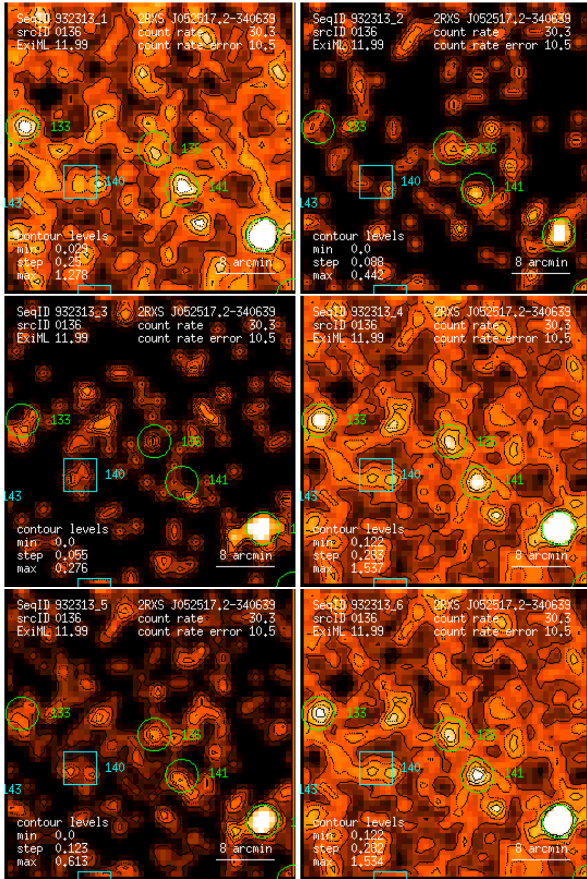
Figure 136: RASS 932313: detection 0136: band rate images, Gaussian filter: (1) PSPC channels 11 – 41, (2) 52 – 90, (3) 91 – 201, (4) 11 – 235, (5) 52 – 201, (6) 11 – 201. Broad band rates in counts/ks. Band rate contour levels in counts/ks/arcmin 2 .
