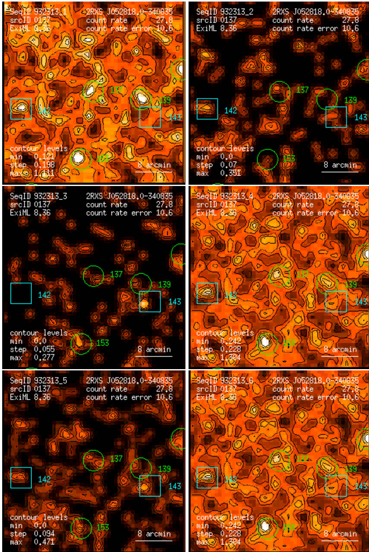
Figure 137: RASS 932313: detection 0137: band rate images, Gaussian filter: (1) PSPC channels 11 – 41, (2) 52 – 90, (3) 91 – 201, (4) 11 – 235, (5) 52 – 201, (6) 11 – 201. Broad band rates in counts/ks. Band rate contour levels in counts/ks/arcmin 2 .
