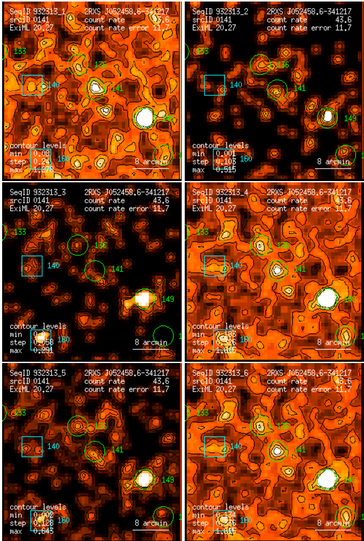
Figure 141: RASS 932313: detection 0141: band rate images, Gaussian filter: (1) PSPC channels 11 – 41, (2) 52 – 90, (3) 91 – 201, (4) 11 – 235, (5) 52 – 201, (6) 11 – 201. Broad band rates in counts/ks. Band rate contour levels in counts/ks/arcmin 2 .
