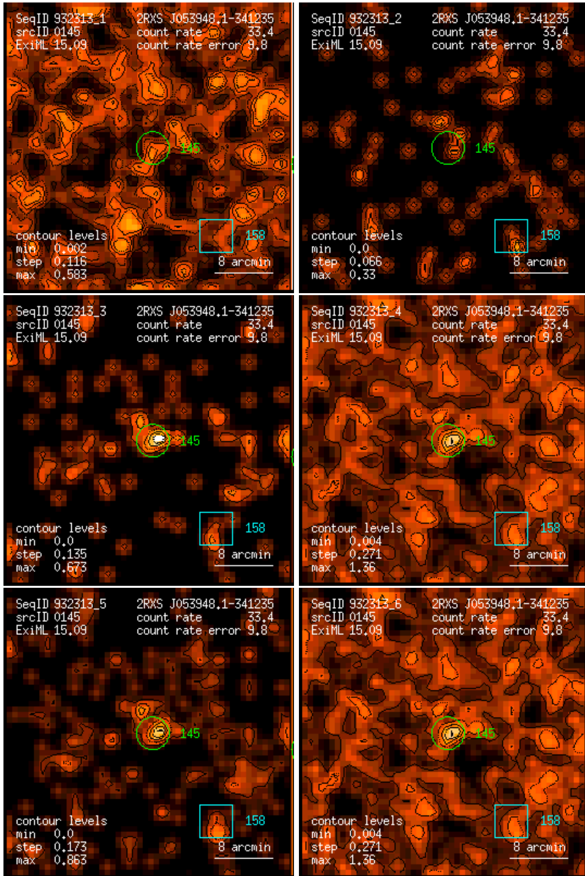
Figure 145: RASS 932313: detection 0145: band rate images, Gaussian filter: (1) PSPC channels 11 – 41, (2) 52 – 90, (3) 91 – 201, (4) 11 – 235, (5) 52 – 201, (6) 11 – 201. Broad band rates in counts/ks. Band rate contour levels in counts/ks/arcmin 2 .
