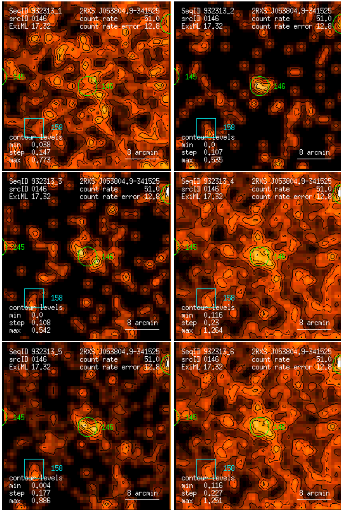
Figure 146: RASS 932313: detection 0146: band rate images, Gaussian filter: (1) PSPC channels 11 – 41, (2) 52 – 90, (3) 91 – 201, (4) 11 – 235, (5) 52 – 201, (6) 11 – 201. Broad band rates in counts/ks. Band rate contour levels in counts/ks/arcmin 2 .
