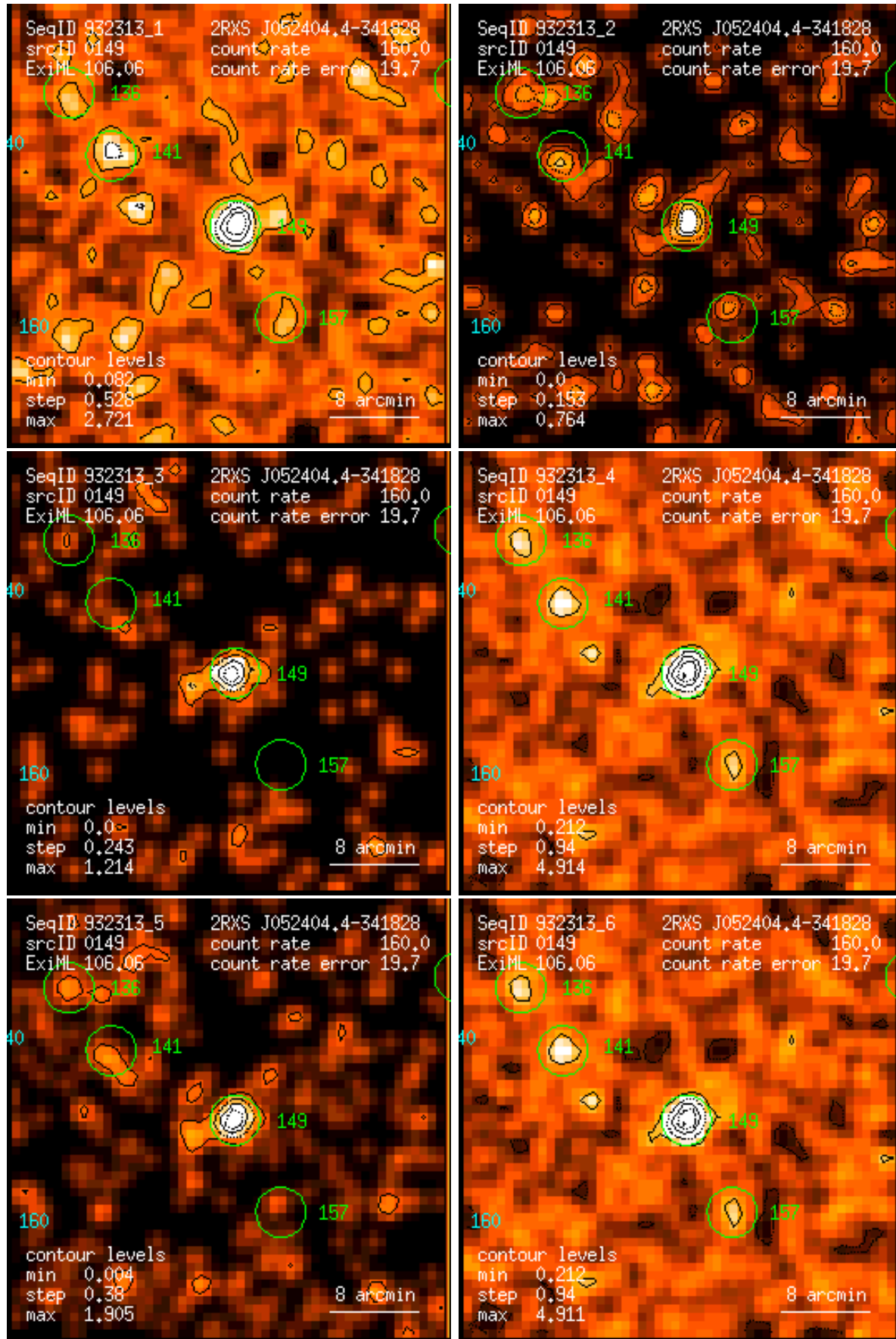
Figure 149: RASS 932313: detection 0149: band rate images, Gaussian filter: (1) PSPC channels 11 – 41, (2) 52 – 90, (3) 91 – 201, (4) 11 – 235, (5) 52 – 201, (6) 11 – 201. Broad band rates in counts/ks. Band rate contour levels in counts/ks/arcmin 2 .
