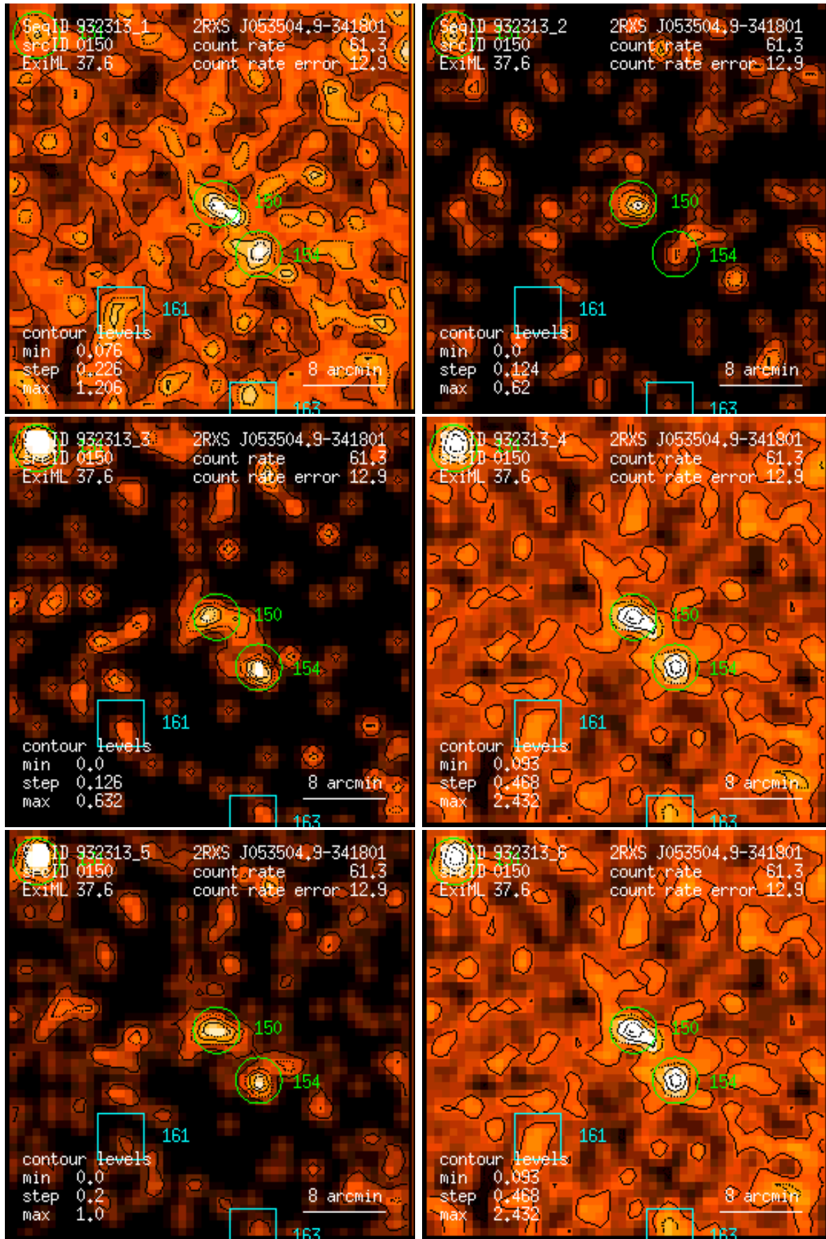
Figure 150: RASS 932313: detection 0150: band rate images, Gaussian filter: (1) PSPC channels 11 – 41, (2) 52 – 90, (3) 91 – 201, (4) 11 – 235, (5) 52 – 201, (6) 11 – 201. Broad band rates in counts/ks. Band rate contour levels in counts/ks/arcmin 2 .
