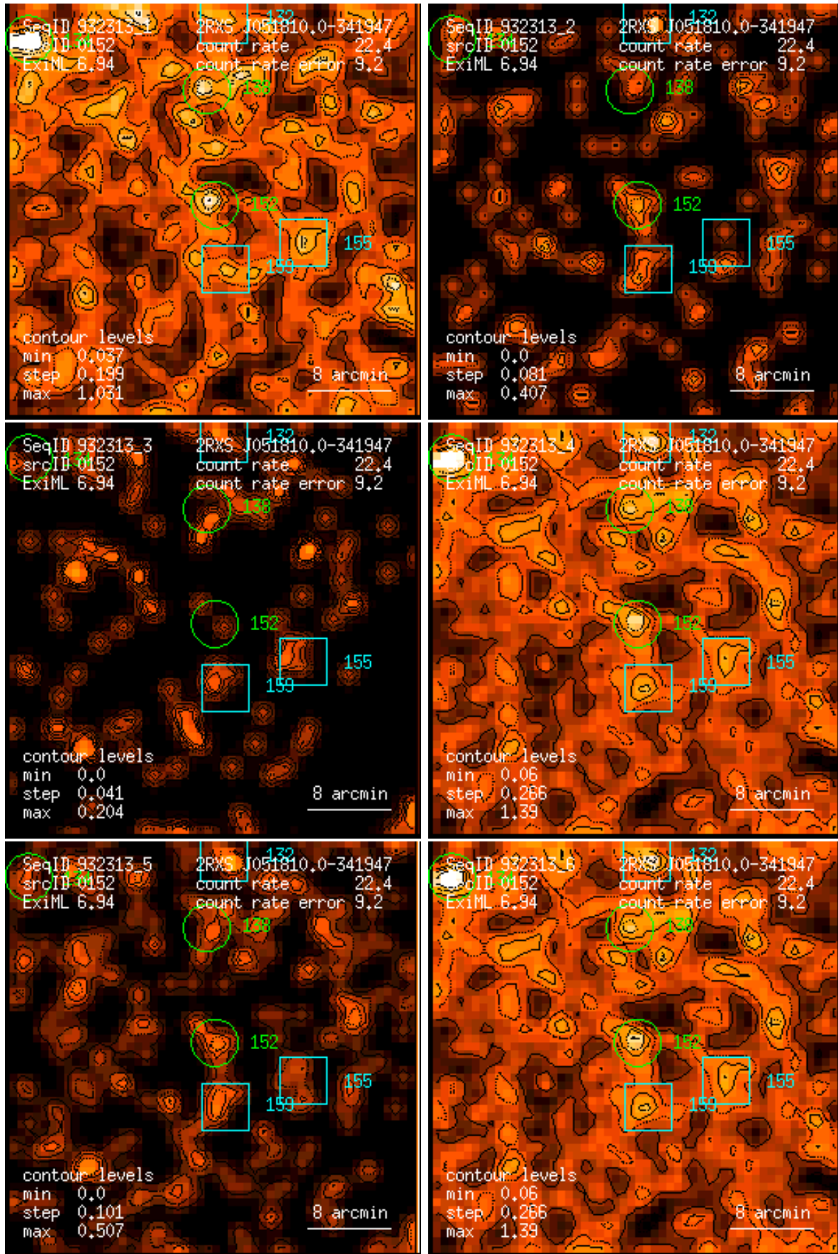
Figure 152: RASS 932313: detection 0152: band rate images, Gaussian filter: (1) PSPC channels 11 – 41, (2) 52 – 90, (3) 91 – 201, (4) 11 – 235, (5) 52 – 201, (6) 11 – 201. Broad band rates in counts/ks. Band rate contour levels in counts/ks/arcmin 2 .
