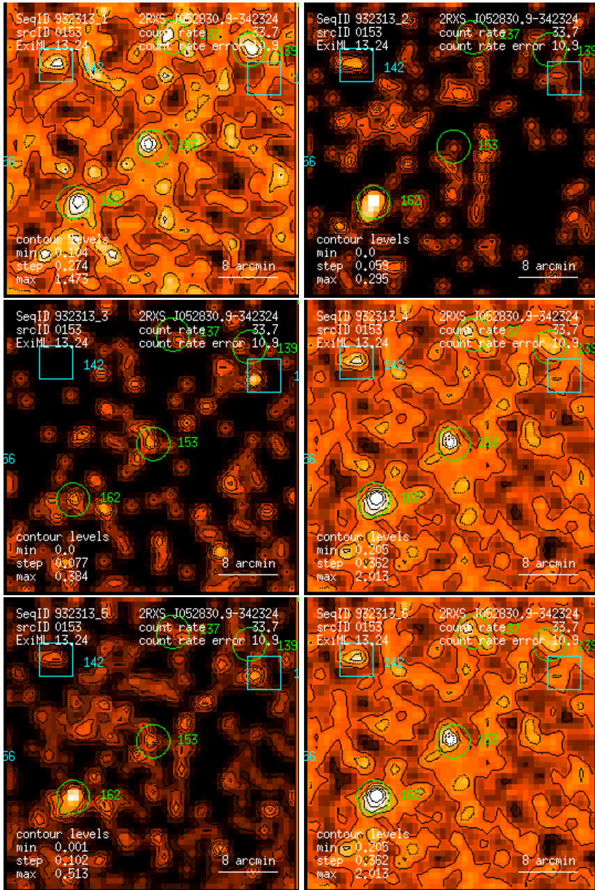
Figure 153: RASS 932313: detection 0153: band rate images, Gaussian filter: (1) PSPC channels 11 – 41, (2) 52 – 90, (3) 91 – 201, (4) 11 – 235, (5) 52 – 201, (6) 11 – 201. Broad band rates in counts/ks. Band rate contour levels in counts/ks/arcmin 2 .
