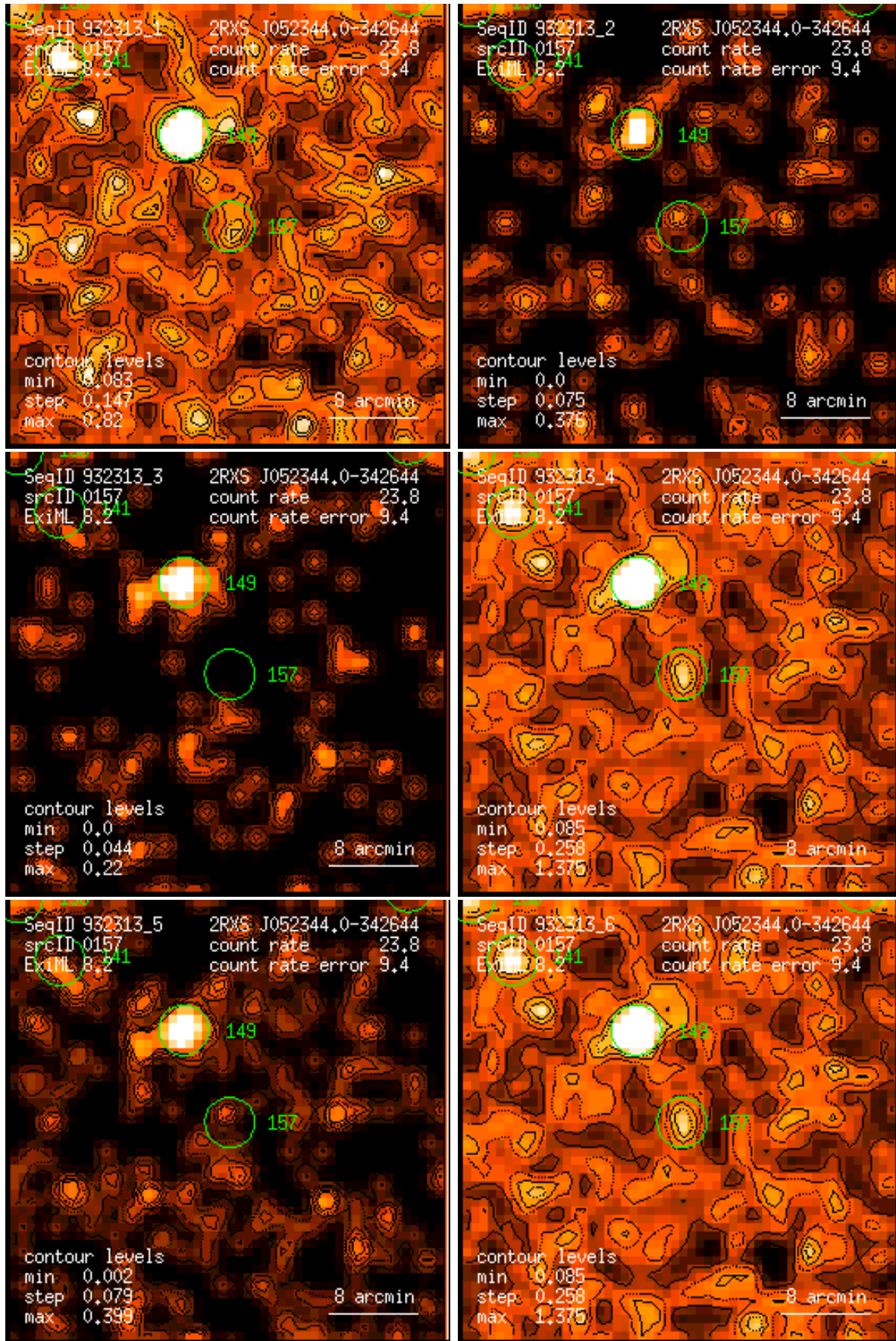
Figure 157: RASS 932313: detection 0157: band rate images, Gaussian filter: (1) PSPC channels 11 – 41, (2) 52 – 90, (3) 91 – 201, (4) 11 – 235, (5) 52 – 201, (6) 11 – 201. Broad band rates in counts/ks. Band rate contour levels in counts/ks/arcmin 2 .
