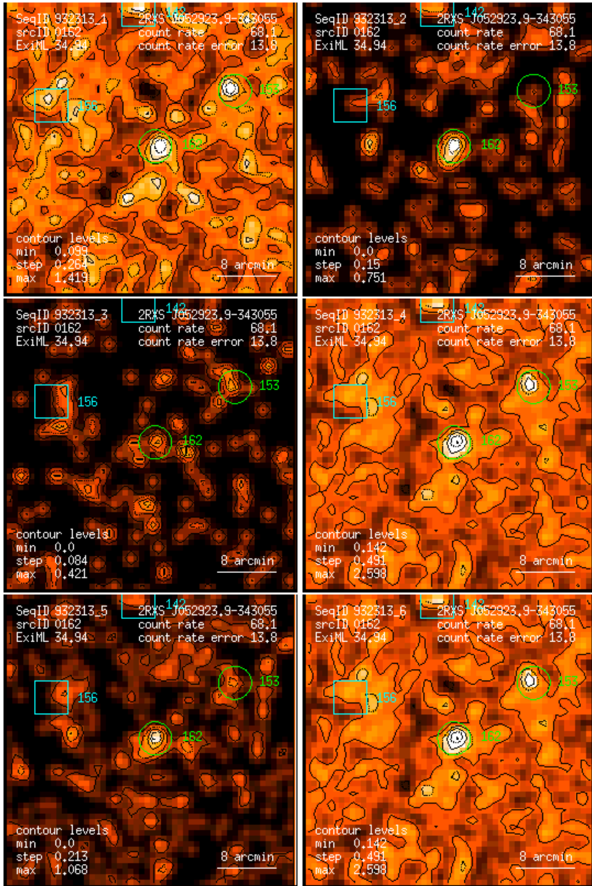
Figure 162: RASS 932313: detection 0162: band rate images, Gaussian filter: (1) PSPC channels 11 – 41, (2) 52 – 90, (3) 91 – 201, (4) 11 – 235, (5) 52 – 201, (6) 11 – 201. Broad band rates in counts/ks. Band rate contour levels in counts/ks/arcmin 2 .
