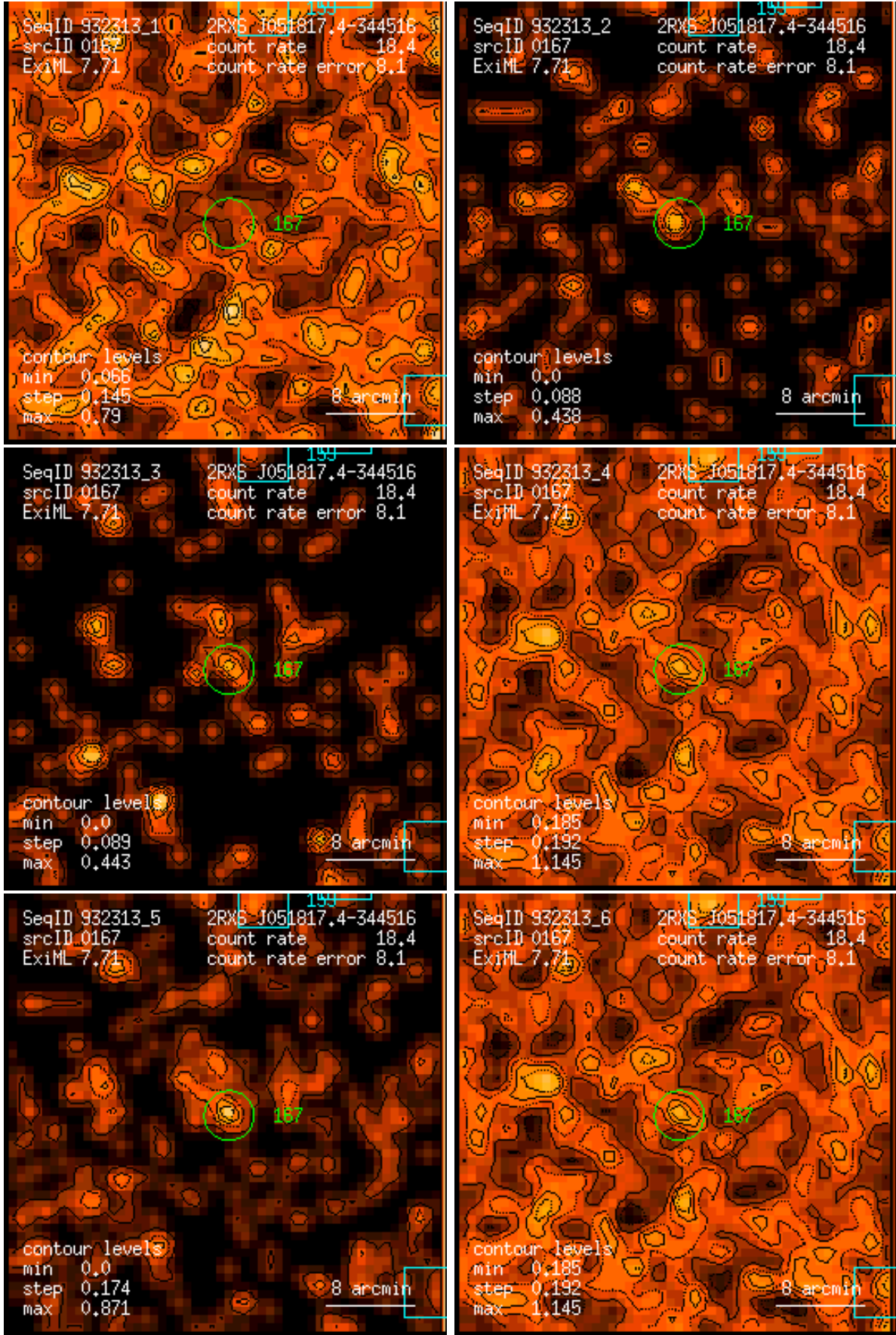
Figure 167: RASS 932313: detection 0167: band rate images, Gaussian filter: (1) PSPC channels 11 – 41, (2) 52 – 90, (3) 91 – 201, (4) 11 – 235, (5) 52 – 201, (6) 11 – 201. Broad band rates in counts/ks. Band rate contour levels in counts/ks/arcmin 2 .
