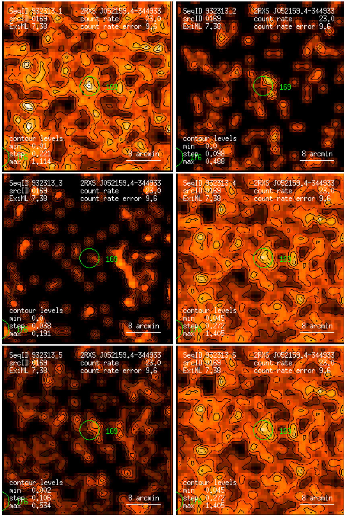
Figure 169: RASS 932313: detection 0169: band rate images, Gaussian filter: (1) PSPC channels 11 – 41, (2) 52 – 90, (3) 91 – 201, (4) 11 – 235, (5) 52 – 201, (6) 11 – 201. Broad band rates in counts/ks. Band rate contour levels in counts/ks/arcmin 2 .
