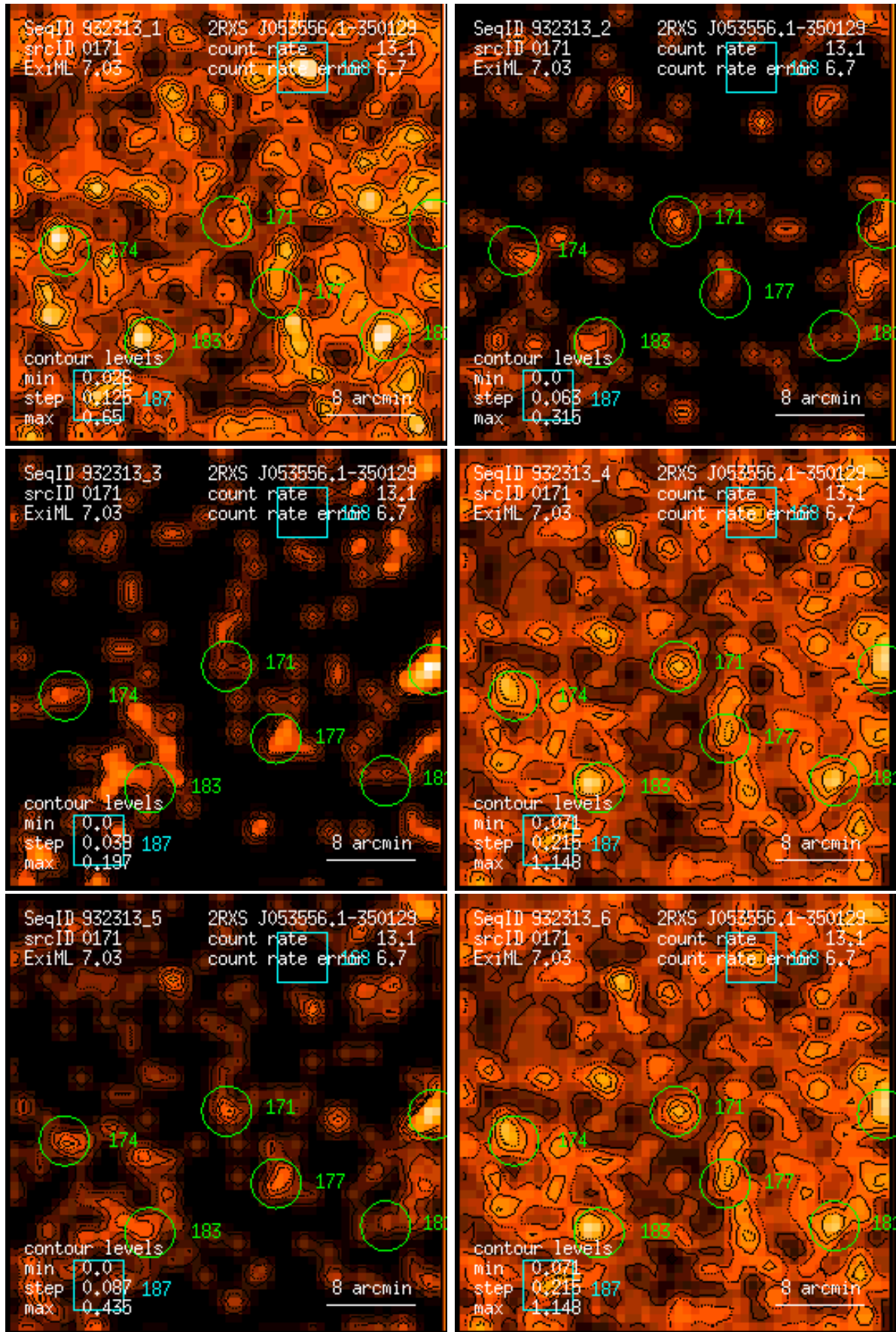
Figure 171: RASS 932313: detection 0171: band rate images, Gaussian filter: (1) PSPC channels 11 – 41, (2) 52 – 90, (3) 91 – 201, (4) 11 – 235, (5) 52 – 201, (6) 11 – 201. Broad band rates in counts/ks. Band rate contour levels in counts/ks/arcmin 2 .
