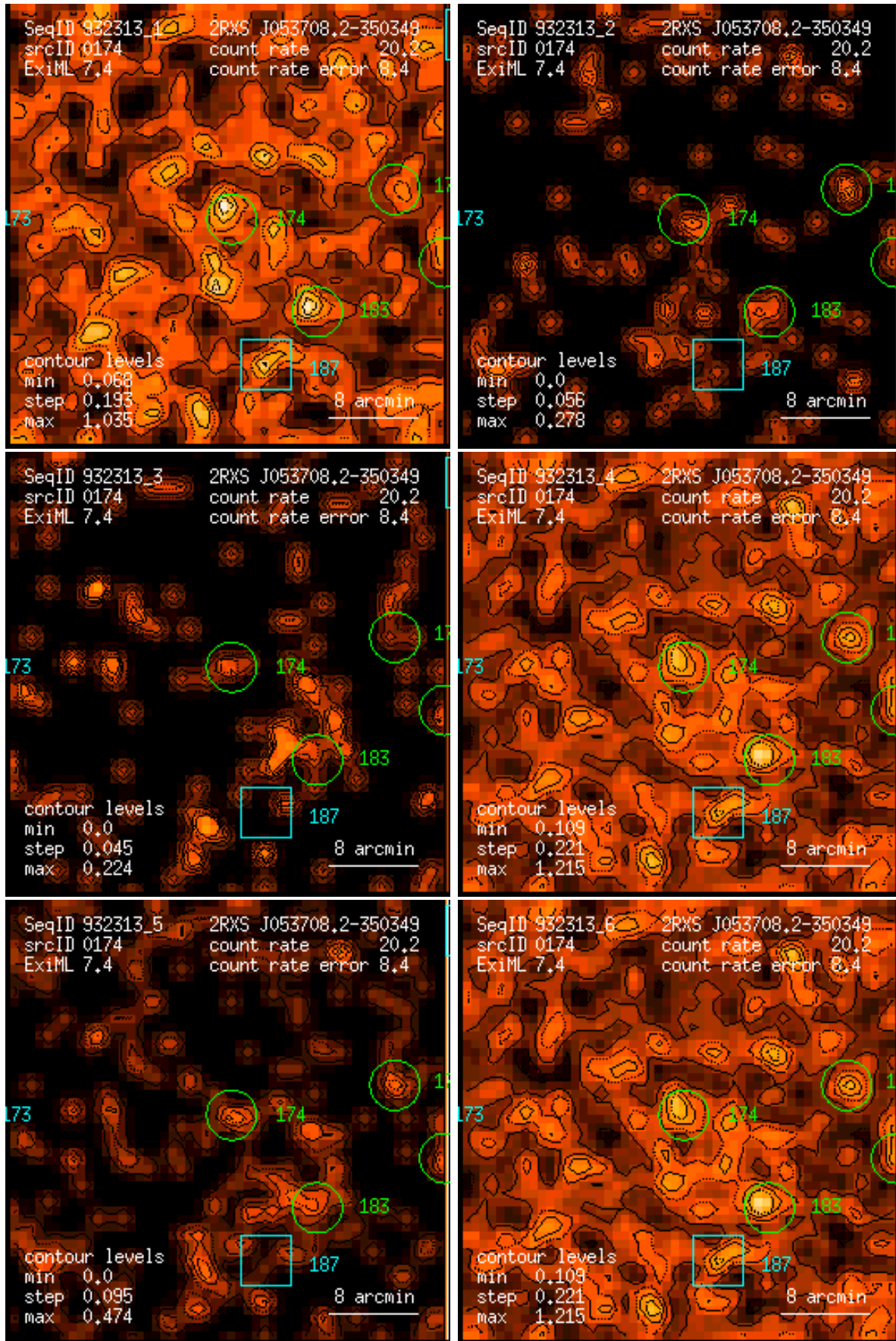
Figure 174: RASS 932313: detection 0174: band rate images, Gaussian filter: (1) PSPC channels 11 – 41, (2) 52 – 90, (3) 91 – 201, (4) 11 – 235, (5) 52 – 201, (6) 11 – 201. Broad band rates in counts/ks. Band rate contour levels in counts/ks/arcmin 2 .
