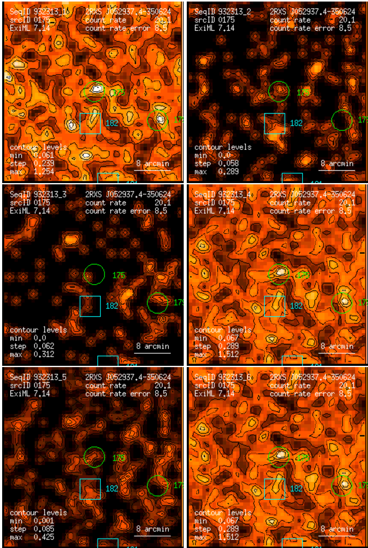
Figure 175: RASS 932313: detection 0175: band rate images, Gaussian filter: (1) PSPC channels 11 – 41, (2) 52 – 90, (3) 91 – 201, (4) 11 – 235, (5) 52 – 201, (6) 11 – 201. Broad band rates in counts/ks. Band rate contour levels in counts/ks/arcmin 2 .
