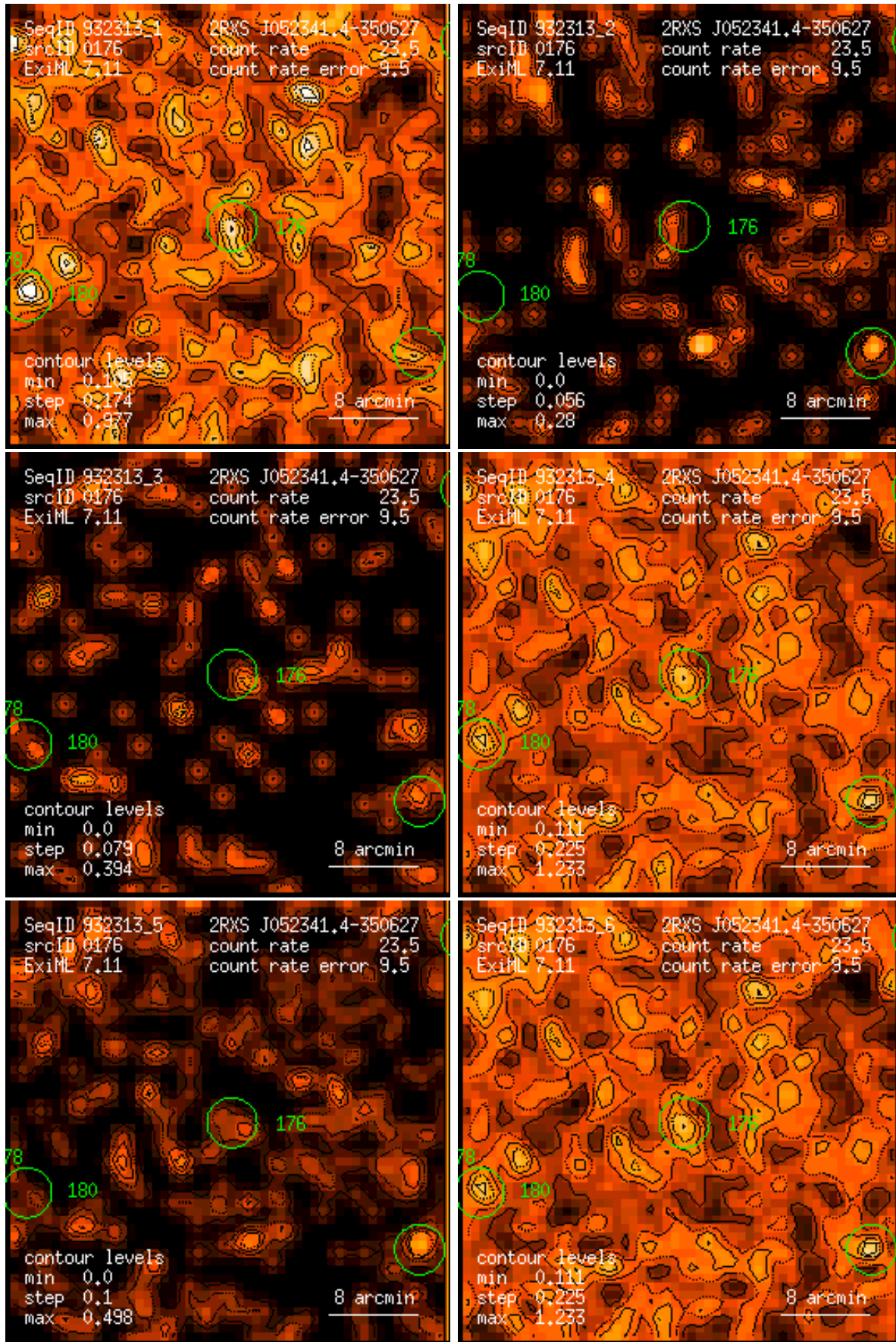
Figure 176: RASS 932313: detection 0176: band rate images, Gaussian filter: (1) PSPC channels 11 – 41, (2) 52 – 90, (3) 91 – 201, (4) 11 – 235, (5) 52 – 201, (6) 11 – 201. Broad band rates in counts/ks. Band rate contour levels in counts/ks/arcmin 2 .
