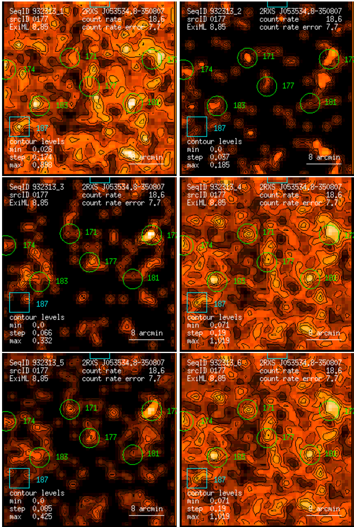
Figure 177: RASS 932313: detection 0177: band rate images, Gaussian filter: (1) PSPC channels 11 – 41, (2) 52 – 90, (3) 91 – 201, (4) 11 – 235, (5) 52 – 201, (6) 11 – 201. Broad band rates in counts/ks. Band rate contour levels in counts/ks/arcmin 2 .
