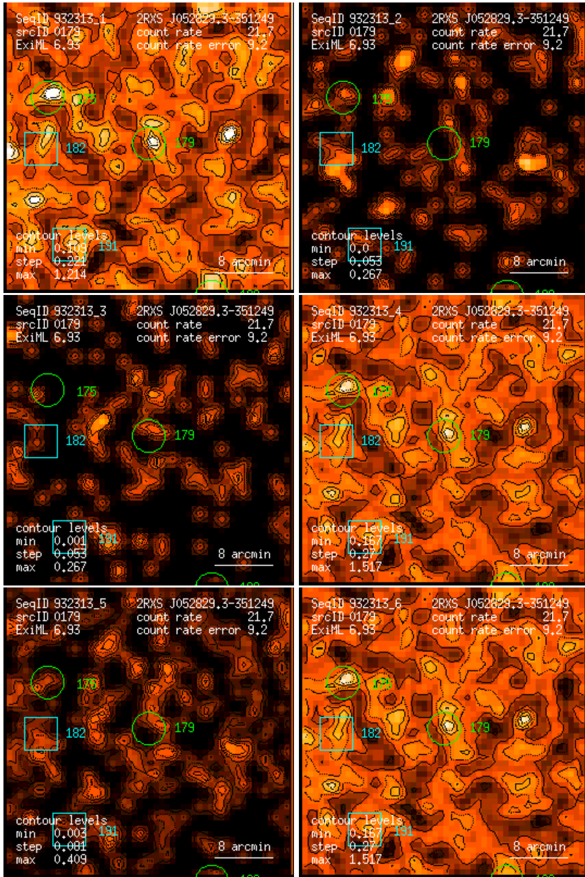
Figure 179: RASS 932313: detection 0179: band rate images, Gaussian filter: (1) PSPC channels 11 – 41, (2) 52 – 90, (3) 91 – 201, (4) 11 – 235, (5) 52 – 201, (6) 11 – 201. Broad band rates in counts/ks. Band rate contour levels in counts/ks/arcmin 2 .
