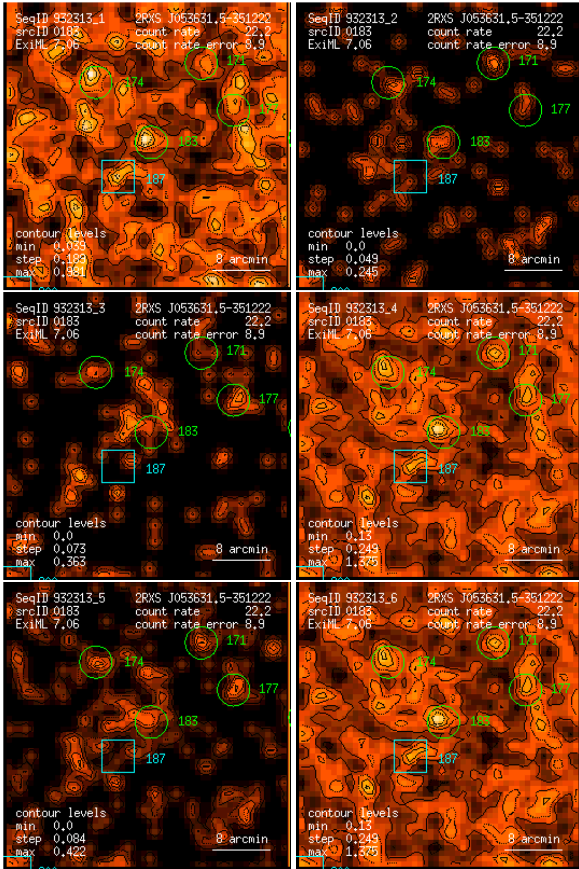
Figure 183: RASS 932313: detection 0183: band rate images, Gaussian filter: (1) PSPC channels 11 – 41, (2) 52 – 90, (3) 91 – 201, (4) 11 – 235, (5) 52 – 201, (6) 11 – 201. Broad band rates in counts/ks. Band rate contour levels in counts/ks/arcmin 2 .
