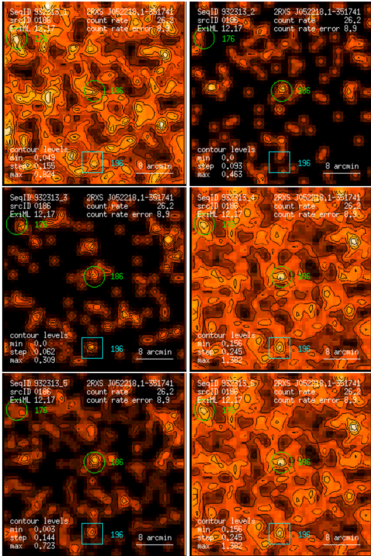
Figure 186: RASS 932313: detection 0186: band rate images, Gaussian filter: (1) PSPC channels 11 – 41, (2) 52 – 90, (3) 91 – 201, (4) 11 – 235, (5) 52 – 201, (6) 11 – 201. Broad band rates in counts/ks. Band rate contour levels in counts/ks/arcmin 2 .
