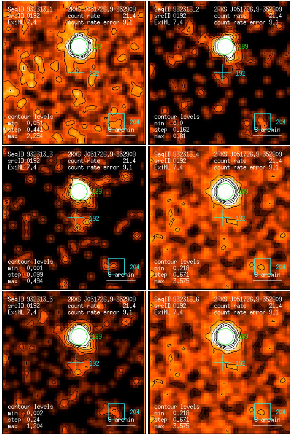
Figure 192: RASS 932313: detection 0192: band rate images, Gaussian filter: (1) PSPC channels 11 – 41, (2) 52 – 90, (3) 91 – 201, (4) 11 – 235, (5) 52 – 201, (6) 11 – 201. Broad band rates in counts/ks. Band rate contour levels in counts/ks/arcmin 2 .
