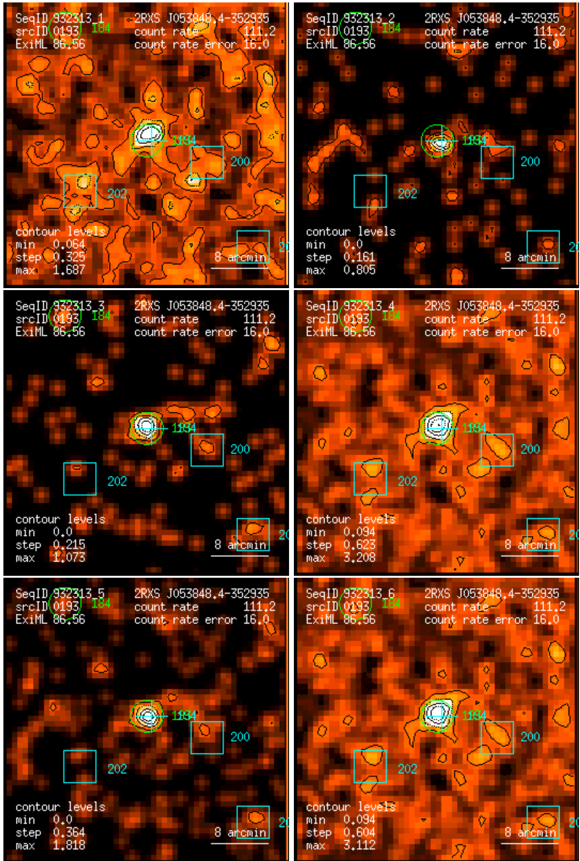
Figure 193: RASS 932313: detection 0193: band rate images, Gaussian filter: (1) PSPC channels 11 – 41, (2) 52 – 90, (3) 91 – 201, (4) 11 – 235, (5) 52 – 201, (6) 11 – 201. Broad band rates in counts/ks. Band rate contour levels in counts/ks/arcmin 2 .
