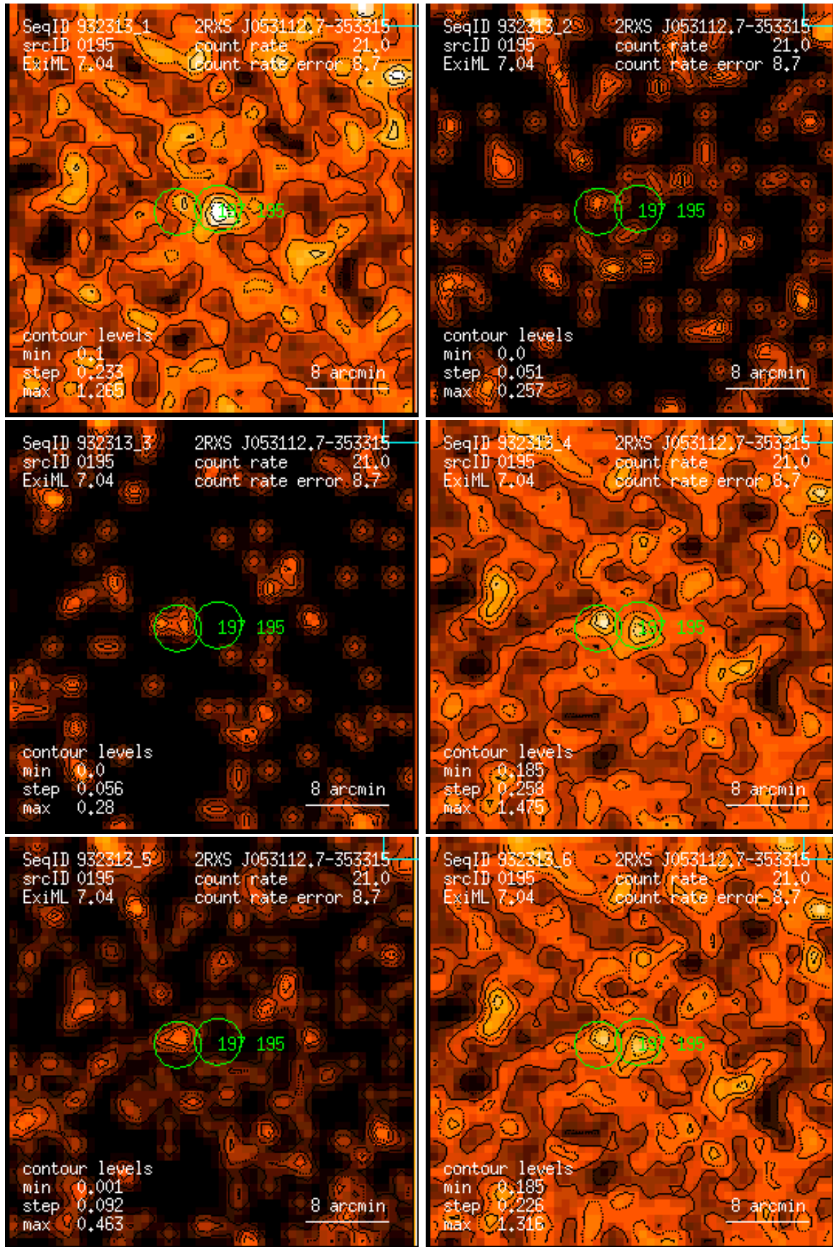
Figure 195: RASS 932313: detection 0195: band rate images, Gaussian filter: (1) PSPC channels 11 – 41, (2) 52 – 90, (3) 91 – 201, (4) 11 – 235, (5) 52 – 201, (6) 11 – 201. Broad band rates in counts/ks. Band rate contour levels in counts/ks/arcmin 2 .
