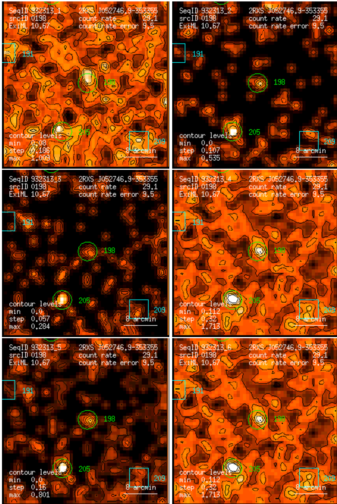
Figure 198: RASS 932313: detection 0198: band rate images, Gaussian filter: (1) PSPC channels 11 – 41, (2) 52 – 90, (3) 91 – 201, (4) 11 – 235, (5) 52 – 201, (6) 11 – 201. Broad band rates in counts/ks. Band rate contour levels in counts/ks/arcmin 2 .
