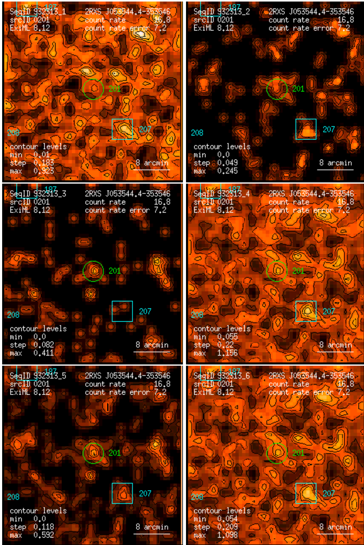
Figure 201: RASS 932313: detection 0201: band rate images, Gaussian filter: (1) PSPC channels 11 – 41, (2) 52 – 90, (3) 91 – 201, (4) 11 – 235, (5) 52 – 201, (6) 11 – 201. Broad band rates in counts/ks. Band rate contour levels in counts/ks/arcmin 2 .
