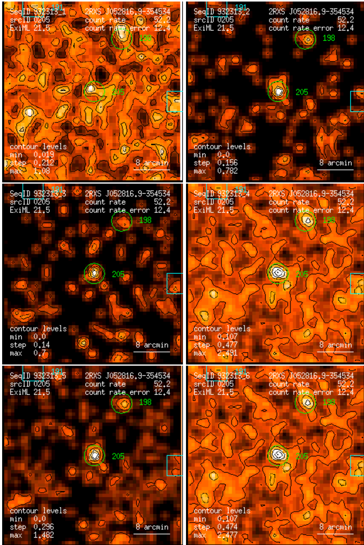
Figure 205: RASS 932313: detection 0205: band rate images, Gaussian filter: (1) PSPC channels 11 – 41, (2) 52 – 90, (3) 91 – 201, (4) 11 – 235, (5) 52 – 201, (6) 11 – 201. Broad band rates in counts/ks. Band rate contour levels in counts/ks/arcmin 2 .
