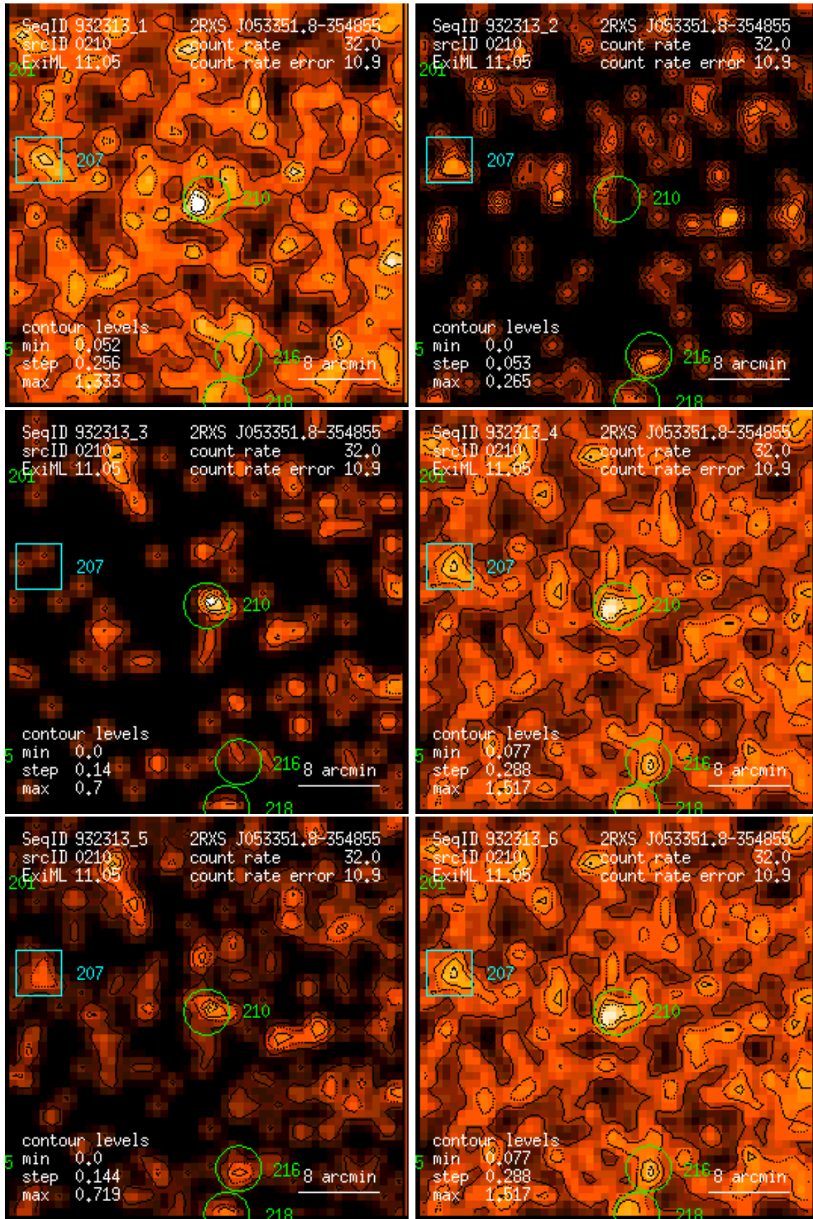
Figure 210: RASS 932313: detection 0210: band rate images, Gaussian filter: (1) PSPC channels 11 – 41, (2) 52 – 90, (3) 91 – 201, (4) 11 – 235, (5) 52 – 201, (6) 11 – 201. Broad band rates in counts/ks. Band rate contour levels in counts/ks/arcmin 2 .
