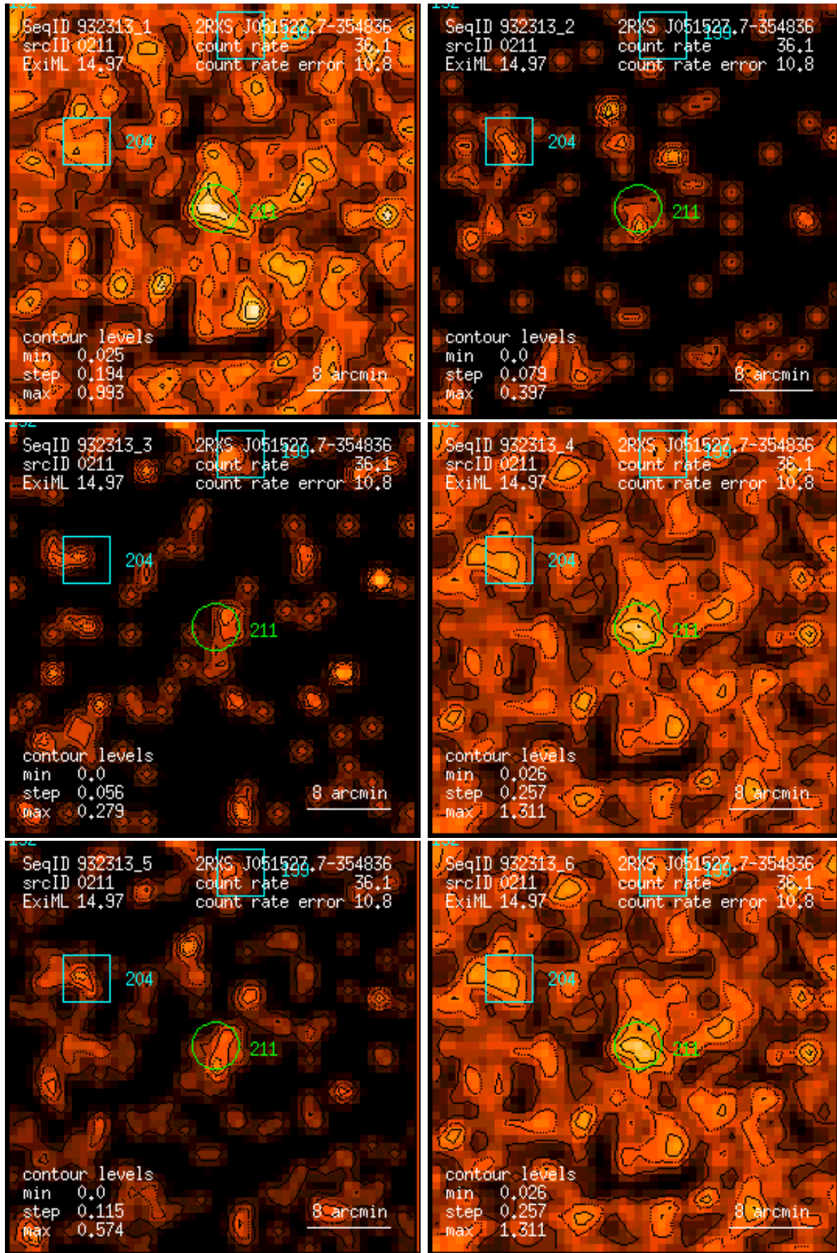
Figure 211: RASS 932313: detection 0211: band rate images, Gaussian filter: (1) PSPC channels 11 – 41, (2) 52 – 90, (3) 91 – 201, (4) 11 – 235, (5) 52 – 201, (6) 11 – 201. Broad band rates in counts/ks. Band rate contour levels in counts/ks/arcmin 2 .
